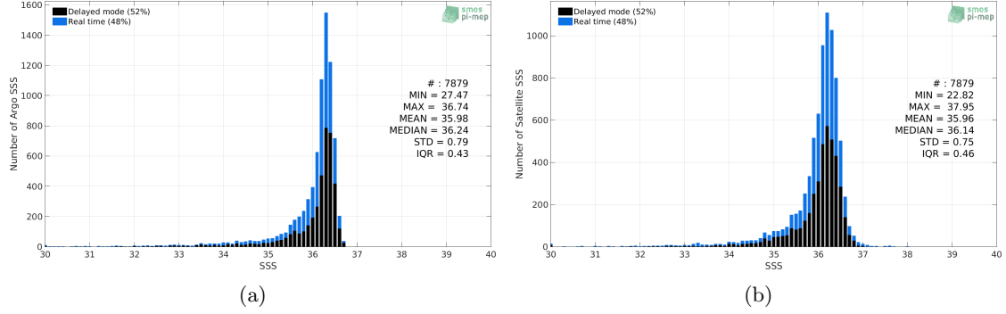
Figure 2: Histograms of SSS from Argo (a) and SMOS SSS L3 v7 - 18 Days (CATDS-CECOS-LOCEAN) (b) considering all match-up pairs per bins of 0.1 over the Mississippi river plume Pi-MEP region and for the full satellite product period.
