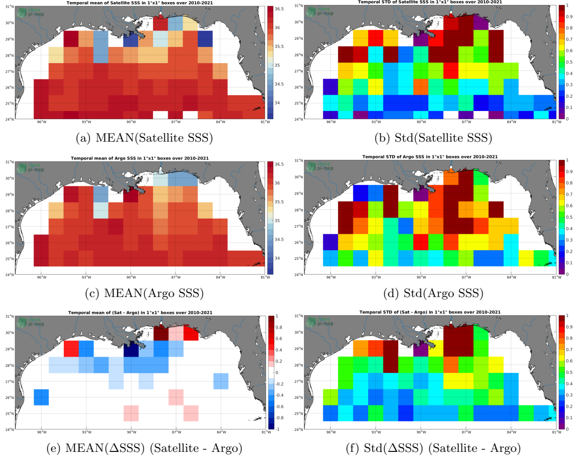
Figure 6: Temporal mean (left) and Std (right) of SSS from SMOS SSS L3 v7 - 18 Days (CATDS-CECOS-LOCEAN) (top), Argo (middle), and of \Delta\text{SSS} (Satellite - Argo). Only match-up pairs are used to generate these maps.
