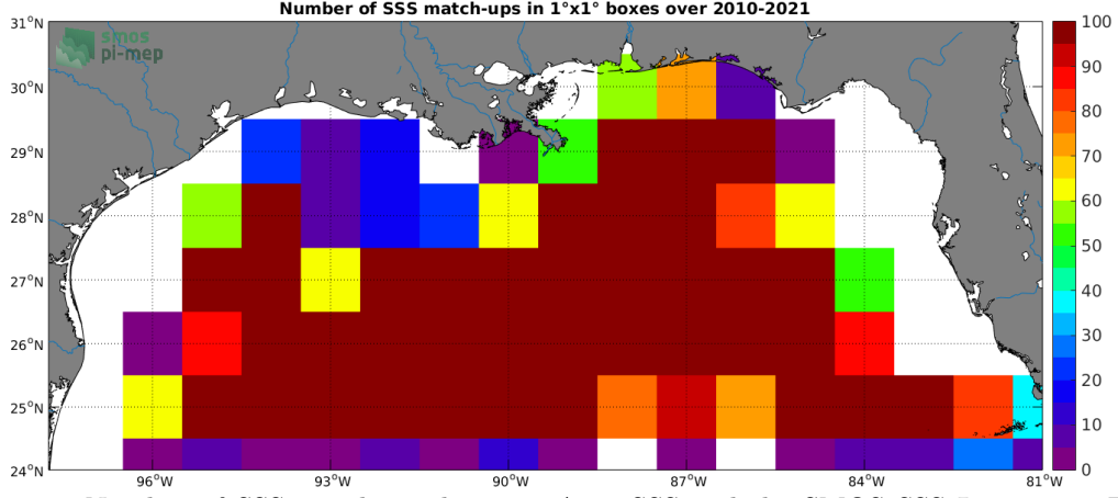
Figure 4: Number of SSS match-ups between Argo SSS and the SMOS SSS L3 v7 - 18 Days (CATDS-CECOS-LOCEAN) SSS product for the Mississippi river plume Pi-MEP region over 1^\circ \times 1^\circ boxes and for the full satellite product period.
