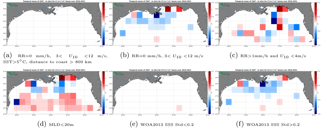
Figure 12: Temporal mean gridded over spatial boxes of size 1^{\circ} \times 1^{\circ} of \Delta\text{SSS} (SMOS SSS L3 v7 - 18 Days (CATDS-CECOS-LOCEAN) - Argo) for 6 different subdatasets corresponding to: \text{RR}=0 mm/h, 3 < U_{10} < 12 m/s, SST > 5^{\circ}\text{C} , distance to coast > 800 km (a), \text{RR}=0 mm/h, 3 < U_{10} < 12 m/s (b), \text{RR} > 1\text{mm/h} and U_{10} < 4\text{m/s} (c), \text{MLD} < 20\text{m} (d), WOA2013 SSS Std < 0.2 (e), WOA2013 SSS Std > 0.2 (f).
