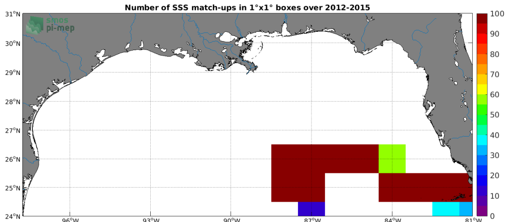
Figure 4: Number of SSS match-ups between TSG (GOSUD-Sailing-ship) SSS and the SMOS SSS L3 v5 - 18 Days (CATDS-CECOS-LOCEAN) SSS product for the Mississippi river plume Pi-MEP region over 1^\circ \times 1^\circ boxes and for the full satellite product period.
