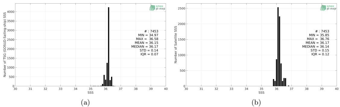
Figure 2: Histograms of SSS from TSG (GOSUD-Sailing-ship) (a) and SMOS SSS L3 v5 - 18 Days (CATDS-CECOS-LOCEAN) (b) considering all match-up pairs per bins of 0.1 over the Mississippi river plume Pi-MEP region and for the full satellite product period.
