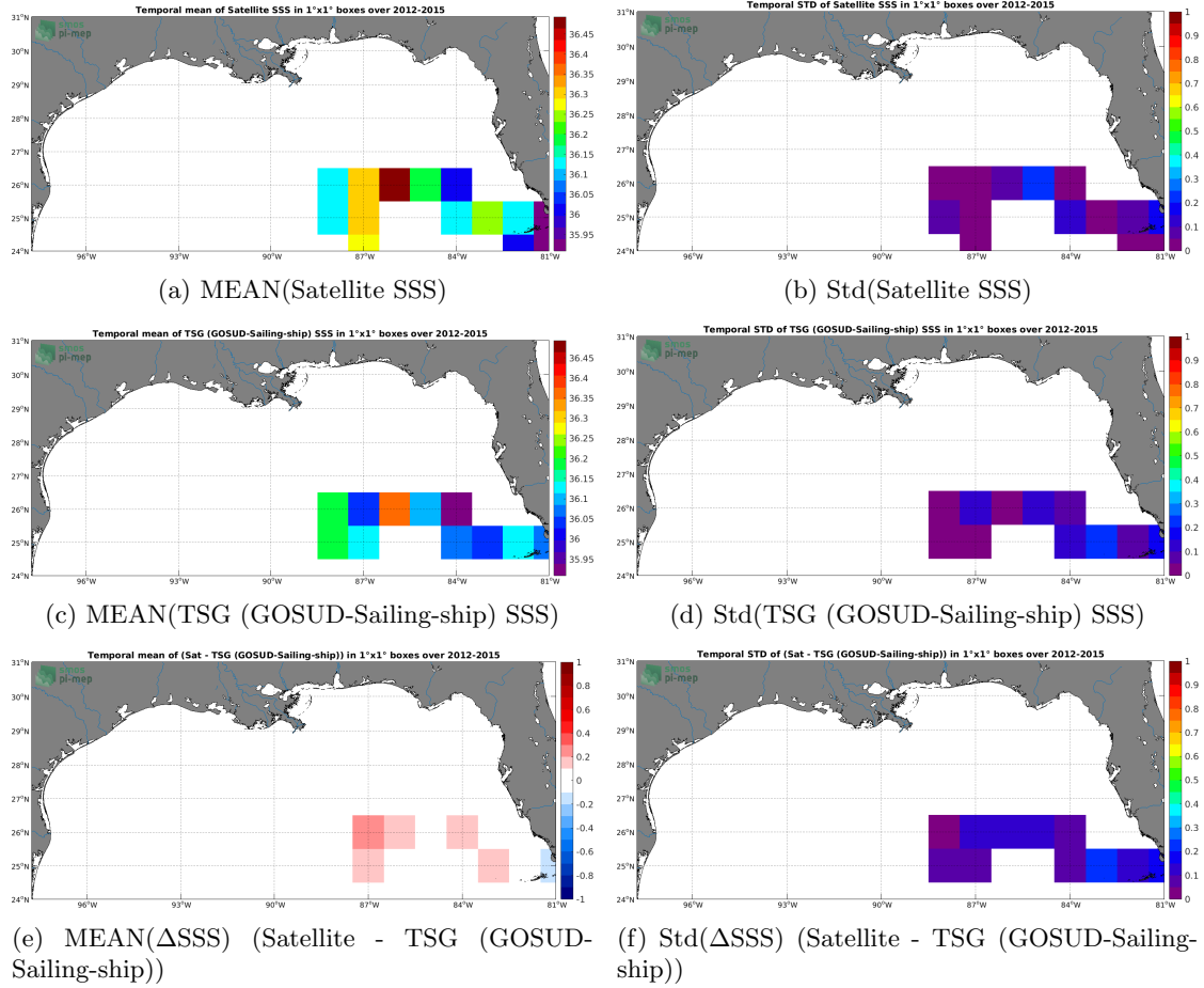
Figure 6: Temporal mean (left) and Std (right) of SSS from SMOS SSS L3 v5 - 18 Days (CATDS-CECOS-LOCEAN) (top), TSG (GOSUD-Sailing-ship) (middle), and of \Delta SSS (Satellite - TSG (GOSUD-Sailing-ship)). Only match-up pairs are used to generate these maps.
