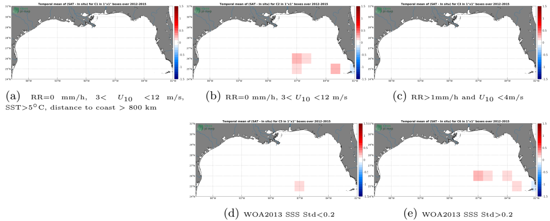
Figure 12: Temporal mean gridded over spatial boxes of size 1^\circ \times 1^\circ of \Delta SSS (SMOS SSS L3 v5 - 18 Days (CATDS-CECOS-LOCEAN) - TSG (GOSUD-Sailing-ship)) for 5 different subdatasets corresponding to: RR=0 mm/h, 3 < U_{10} < 12 m/s, SST > 5^\circ\text{C} , distance to coast > 800 km (a), RR=0 mm/h, 3 < U_{10} < 12 m/s (b), RR > 1 mm/h and U_{10} < 4 m/s (c), WOA2013 SSS Std < 0.2 (d), WOA2013 SSS Std > 0.2 (e).
