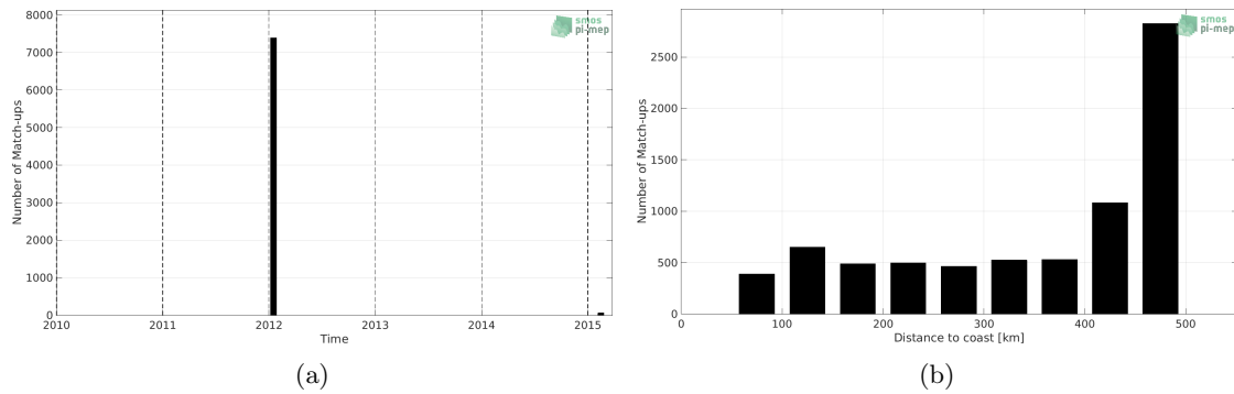
Figure 1: Number of match-ups between TSG (GOSUD-Sailing-ship) and SMOS SSS L3 v5 - 18 Days (CATDS-CECOS-LOCEAN) SSS as a function of time (a) and as function of the distance to coast (b) over the Mississippi river plume Pi-MEP region and for the full satellite product period.
