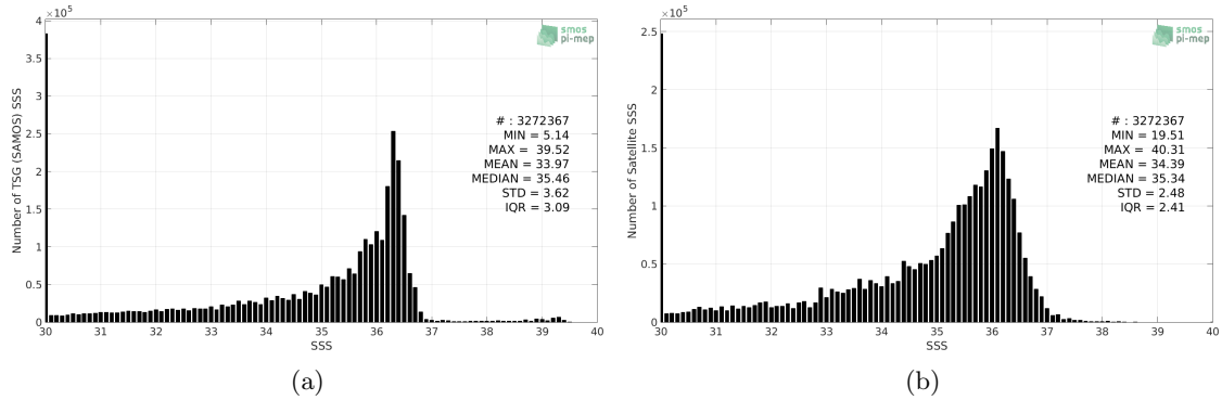
Figure 2: Histograms of SSS from TSG (SAMOS) (a) and SMOS SSS L3 v4 - 9 Days (CATDS-CECOS-LOCEAN) (b) considering all match-up pairs per bins of 0.1 over the Mississippi river plume Pi-MEP region and for the full satellite product period.
