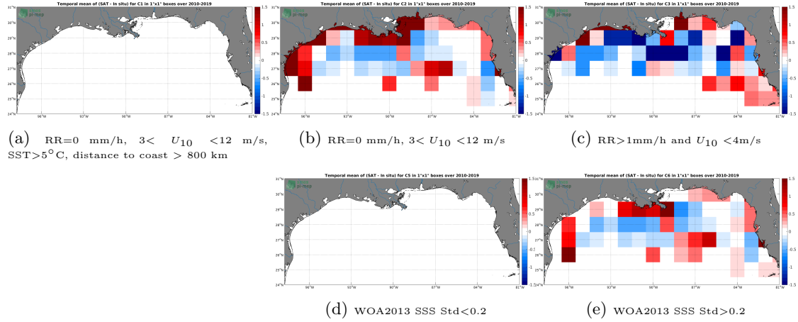
Figure 12: Temporal mean gridded over spatial boxes of size 1^{\circ}\times 1^{\circ} of \Delta\text{SSS} (SMOS SSS L3 v4 - 9 Days (CATDS-CECOS-LOCEAN) - TSG (SAMOS)) for 5 different subdatasets corresponding to:RR=0 mm/h, 3 < U_{10} < 12 m/s, SST >5^{\circ}\text{C} , distance to coast > 800 km (a), RR=0 mm/h, 3 < U_{10} < 12 m/s (b), RR >1 mm/h and U_{10} < 4 m/s (c), WOA2013 SSS Std <0.2 (d), WOA2013 SSS Std >0.2 (e).
