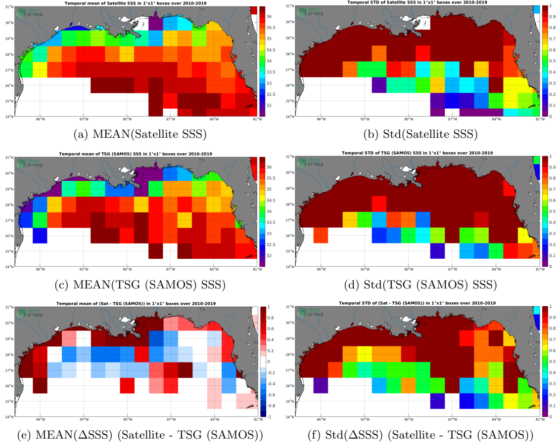
Figure 6: Temporal mean (left) and Std (right) of SSS from SMOS SSS L3 v4 - 9 Days (CATDS-CECOS-LOCEAN) (top), TSG (SAMOS) (middle), and of \Delta SSS (Satellite - TSG (SAMOS)). Only match-up pairs are used to generate these maps.
