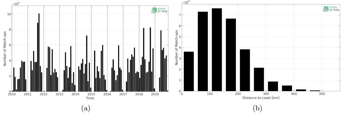
Figure 1: Number of match-ups between TSG (SAMOS) and SMOS SSS L3 v4 - 9 Days (CATDS-CECOS-LOCEAN) SSS as a function of time (a) and as function of the distance to coast (b) over the Mississippi river plume Pi-MEP region and for the full satellite product period.
