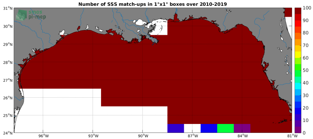
Figure 4: Number of SSS match-ups between TSG (SAMOS) SSS and the SMOS SSS L3 v4 - 9 Days (CATDS-CECOS-LOCEAN) SSS product for the Mississippi river plume Pi-MEP region over 1°x1° boxes and for the full satellite product period.
