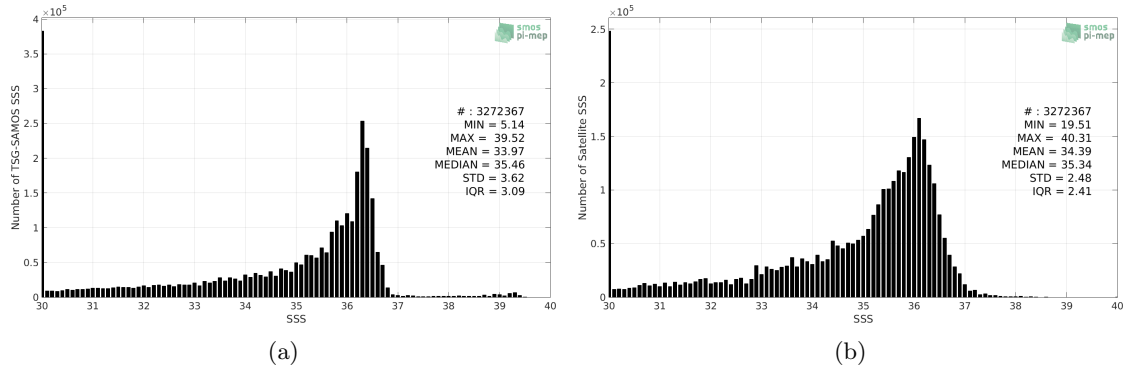
Figure 2: Histograms of SSS from TSG-SAMOS (a) and SMOS-L3-CATDS-CECOS-LOCEAN-V4-9DAYS-25KM (b) considering all match-up pairs per bins of 0.1 over the Mississippi river plume Pi-MEP region and for the full satellite product period.
