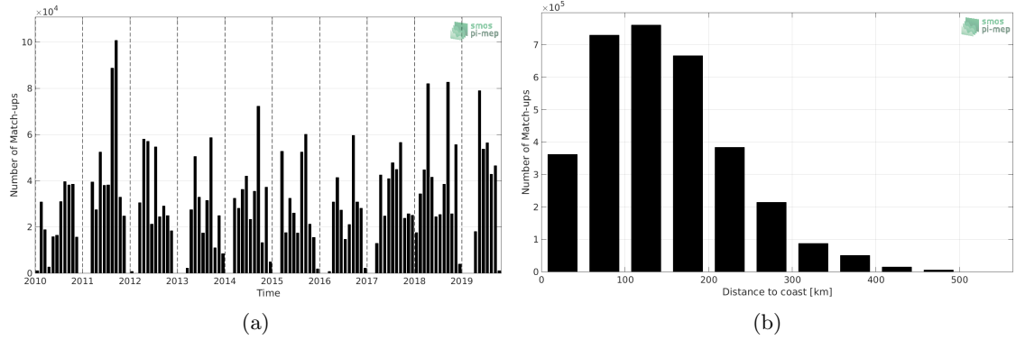
Figure 1: Number of match-ups between TSG-SAMOS and SMOS-L3-CATDS-CECOS-LOCEAN-V4-9DAYS-25KM SSS as a function of time (a) and as function of the distance to coast (b) over the Mississippi river plume Pi-MEP region and for the full satellite product period.
