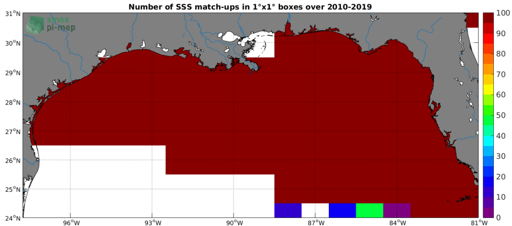
Figure 4: Number of SSS match-ups between TSG-SAMOS SSS and the SMOS-L3-CATDS-CECOS-LOCEAN-V4-9DAYS-25KM SSS product for the Mississippi river plume Pi-MEP region over 1°x1° boxes and for the full satellite product period.
