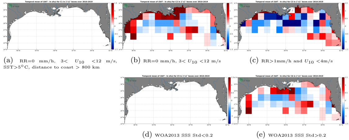
Figure 12: Temporal mean gridded over spatial boxes of size 1^{\circ}\times 1^{\circ} of \Delta\text{SSS} (SMOS-L3-CATDS-CECOS-LOCEAN-V4-9DAYS-25KM - TSG-SAMOS) for 5 different subdatasets corresponding to: RR=0 mm/h, 3 < U_{10} < 12 m/s, SST > 5^{\circ}\text{C} , distance to coast > 800 km (a), RR=0 mm/h, 3 < U_{10} < 12 m/s (b), RR > 1 mm/h and U_{10} < 4 m/s (c), WOA2013 SSS Std < 0.2 (d), WOA2013 SSS Std > 0.2 (e).
