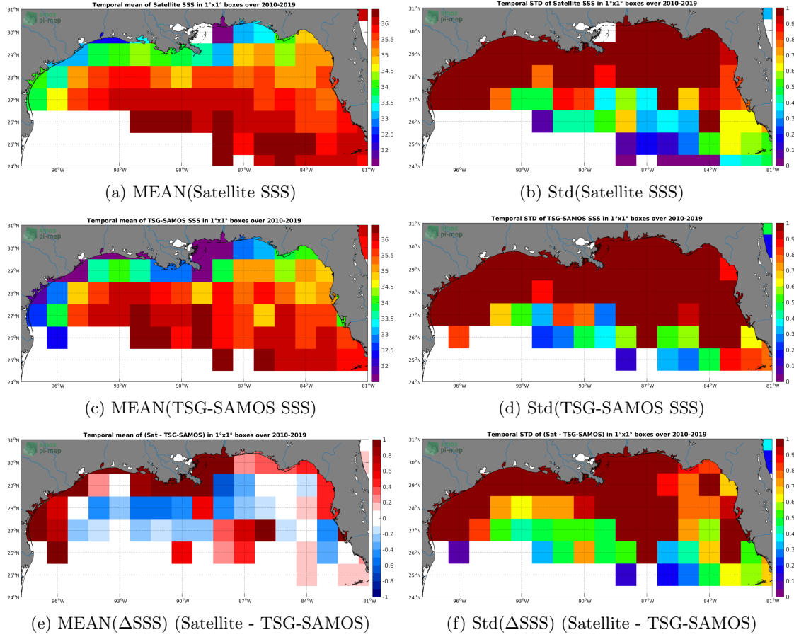
Figure 6: Temporal mean (left) and Std (right) of SSS from SMOS-L3-CATDS-CECOS-LOCEAN-V4-9DAYS-25KM (top), TSG-SAMOS (middle), and of \Delta SSS (Satellite - TSG-SAMOS). Only match-up pairs are used to generate these maps.
