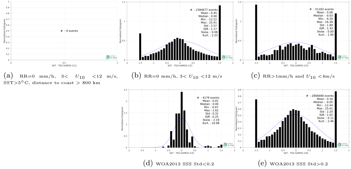
Figure 13: Normalized histogram of \Delta\text{SSS} (SMOS-L3-CATDS-CECOS-LOCEAN-V4-9DAYS-25KM - TSG-SAMOS) for 5 different subdatasets corresponding to: RR=0 mm/h, 3 < U_{10} < 12 m/s, SST >5^{\circ}\text{C} , distance to coast > 800 km (a), RR=0 mm/h, 3 < U_{10} < 12 m/s (b), RR>1\text{mm/h} and U_{10} < 4\text{m/s} (c), WOA2013 SSS Std <0.2 (d), WOA2013 SSS Std >0.2 (e).
