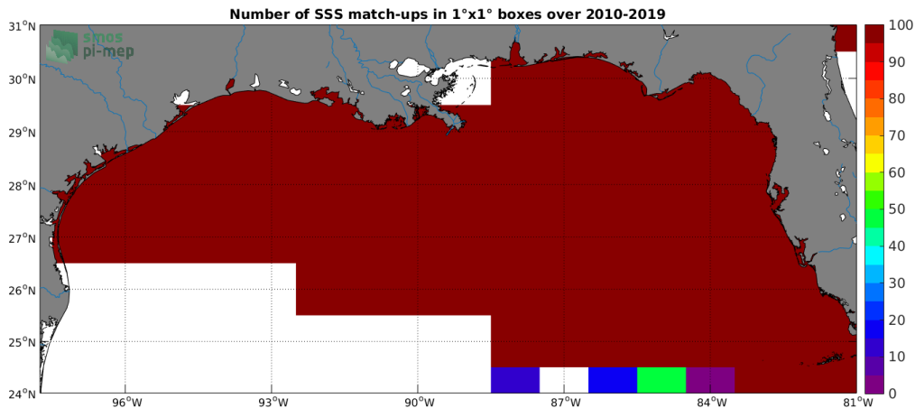
Figure 4: Number of SSS match-ups between TSG (SAMOS) SSS and the SMOS SSS L3 v4 - 18 Days (CATDS-CECOS-LOCEAN) SSS product for the Mississippi river plume Pi-MEP region over 1^\circ \times 1^\circ boxes and for the full satellite product period.
