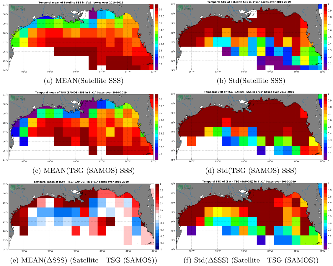
Figure 6: Temporal mean (left) and Std (right) of SSS from SMOS SSS L3 v4 - 18 Days (CATDS-CECOS-LOCEAN) (top), TSG (SAMOS) (middle), and of \Delta SSS (Satellite - TSG (SAMOS)). Only match-up pairs are used to generate these maps.
