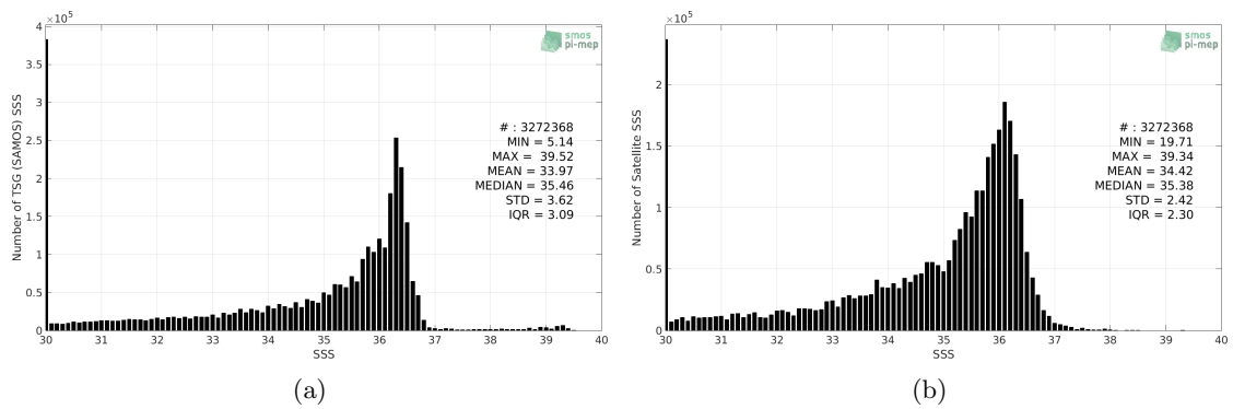
Figure 2: Histograms of SSS from TSG (SAMOS) (a) and SMOS SSS L3 v4 - 18 Days (CATDS-CECOS-LOCEAN) (b) considering all match-up pairs per bins of 0.1 over the Mississippi river plume Pi-MEP region and for the full satellite product period.
