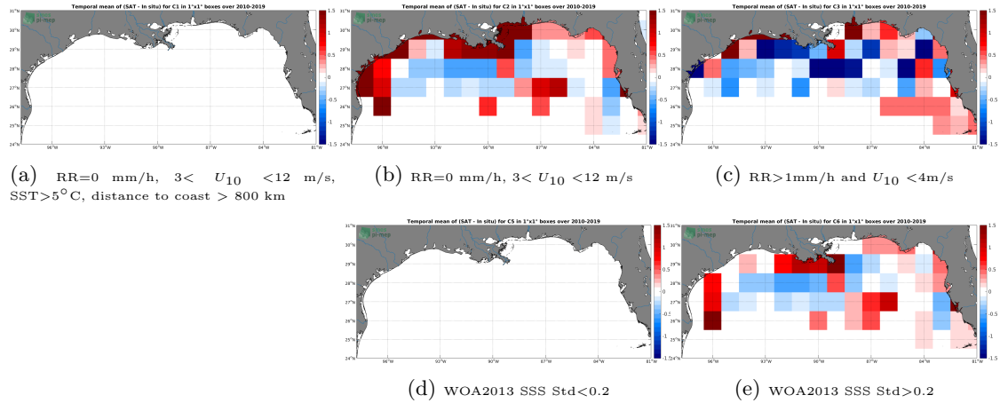
Figure 12: Temporal mean gridded over spatial boxes of size 1^{\circ}\times 1^{\circ} of \Delta\text{SSS} (SMOS SSS L3 v4 - 18 Days (CATDS-CECOS-LOCEAN) - TSG (SAMOS)) for 5 different subdatasets corresponding to:RR=0 mm/h, 3 < U_{10} < 12 m/s, SST >5^{\circ}\text{C} , distance to coast > 800 km (a), RR=0 mm/h, 3 < U_{10} < 12 m/s (b), RR >1 mm/h and U_{10} < 4 m/s (c), WOA2013 SSS Std <0.2 (d), WOA2013 SSS Std >0.2 (e).
