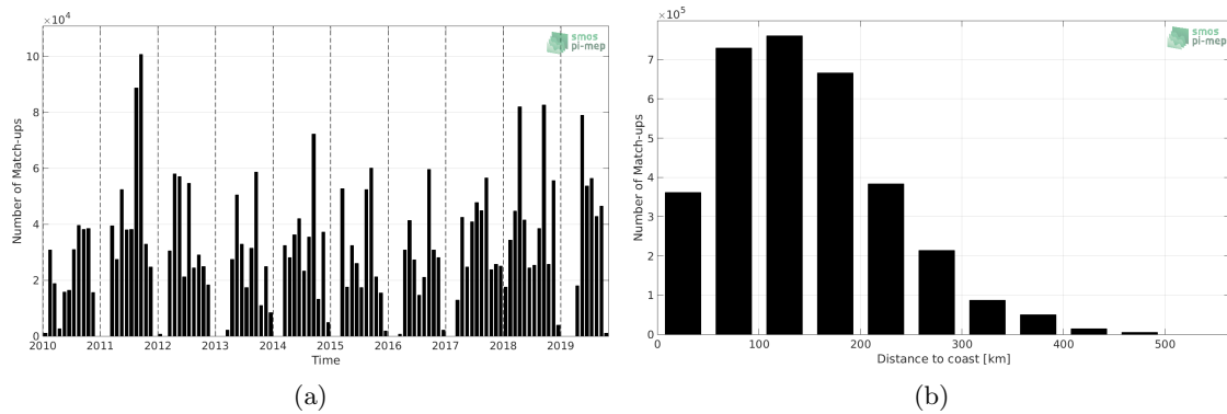
Figure 1: Number of match-ups between TSG (SAMOS) and SMOS SSS L3 v4 - 18 Days (CATDS-CECOS-LOCEAN) SSS as a function of time (a) and as function of the distance to coast (b) over the Mississippi river plume Pi-MEP region and for the full satellite product period.
