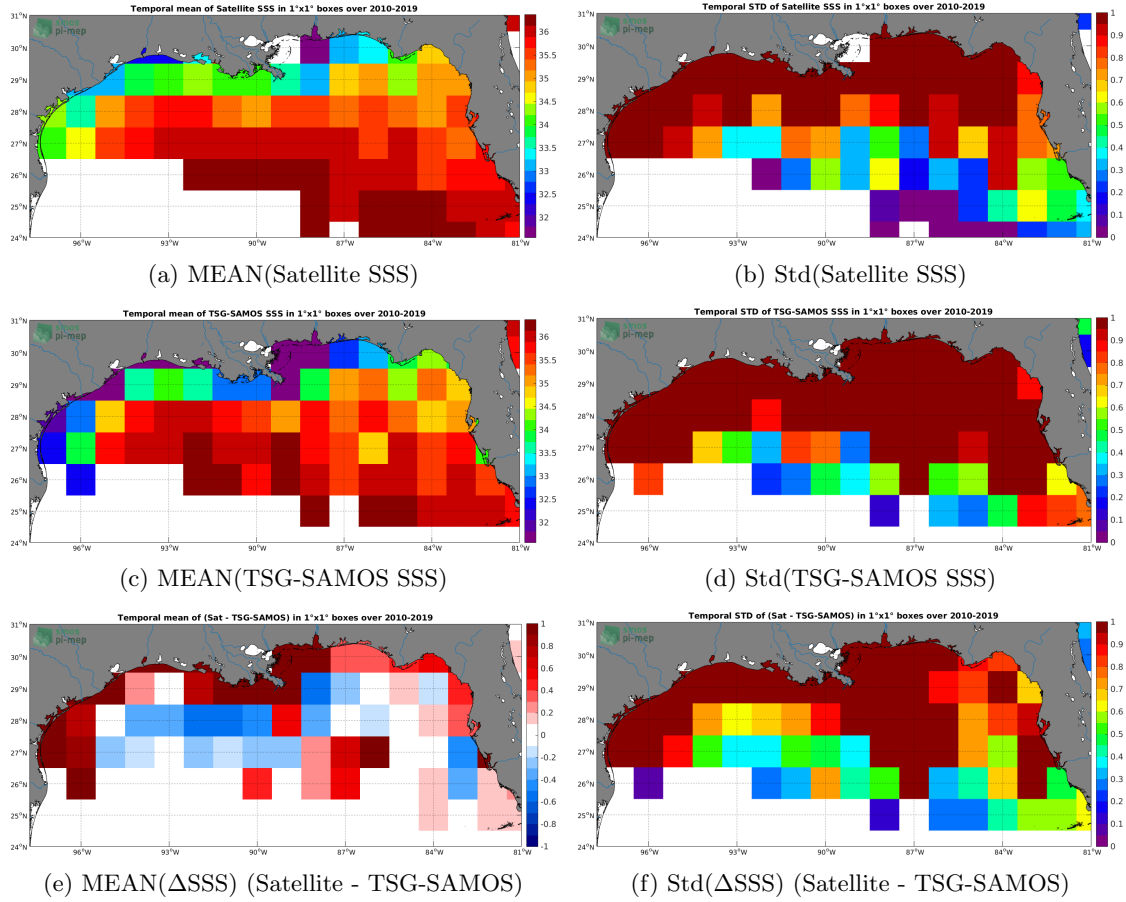
Figure 6: Temporal mean (left) and Std (right) of SSS from SMOS-L3-CATDS-CECOS-LOCEAN-V4-18DAYS-25KM (top), TSG-SAMOS (middle), and of \Delta SSS (Satellite - TSG-SAMOS). Only match-up pairs are used to generate these maps.
