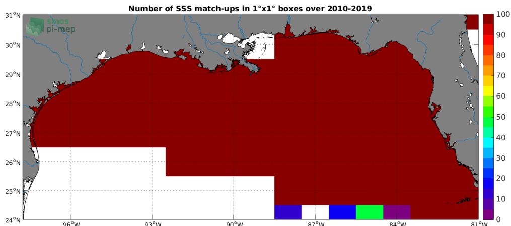
Figure 4: Number of SSS match-ups between TSG-SAMOS SSS and the SMOS-L3-CATDS-CECOS-LOCEAN-V4-18DAYS-25KM SSS product for the Mississippi river plume Pi-MEP region over 1^\circ \times 1^\circ boxes and for the full satellite product period.
