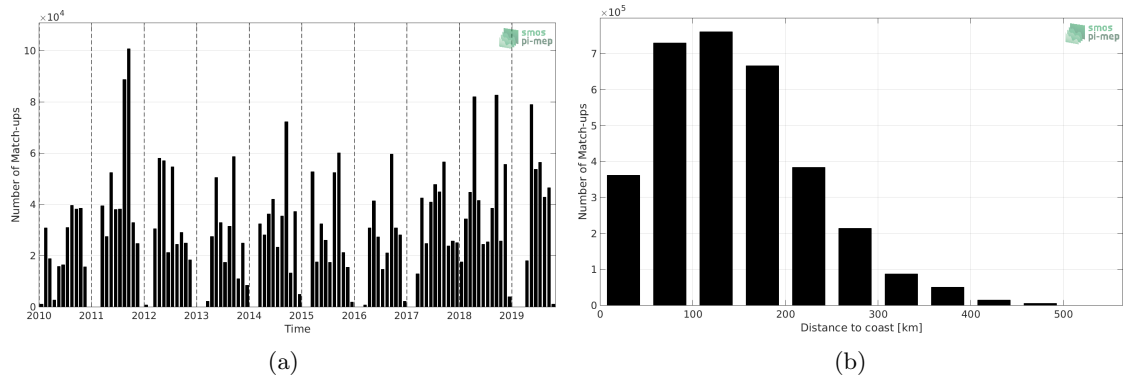
Figure 1: Number of match-ups between TSG-SAMOS and SMOS-L3-CATDS-CECOS-LOCEAN-V4-18DAYS-25KM SSS as a function of time (a) and as function of the distance to coast (b) over the Mississippi river plume Pi-MEP region and for the full satellite product period.
