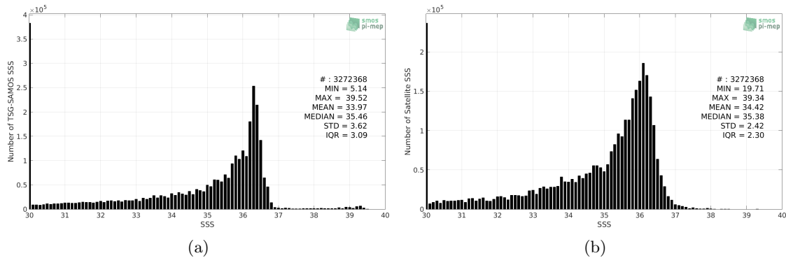
Figure 2: Histograms of SSS from TSG-SAMOS (a) and SMOS-L3-CATDS-CECOS-LOCEAN-V4-18DAYS-25KM (b) considering all match-up pairs per bins of 0.1 over the Mississippi river plume Pi-MEP region and for the full satellite product period.
