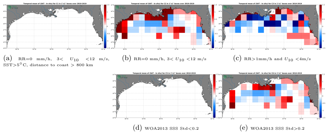
Figure 12: Temporal mean gridded over spatial boxes of size 1^{\circ}\times 1^{\circ} of \Delta\text{SSS} (SMOS-L3-CATDS-CECOS-LOCEAN-V4-18DAYS-25KM - TSG-SAMOS) for 5 different subdatasets corresponding to:RR=0 mm/h, 3 < U_{10} < 12 m/s, SST >5^{\circ}\text{C} , distance to coast > 800 km (a), RR=0 mm/h, 3 < U_{10} < 12 m/s (b), RR >1 mm/h and U_{10} < 4 m/s (c), WOA2013 SSS Std <0.2 (d), WOA2013 SSS Std >0.2 (e).
