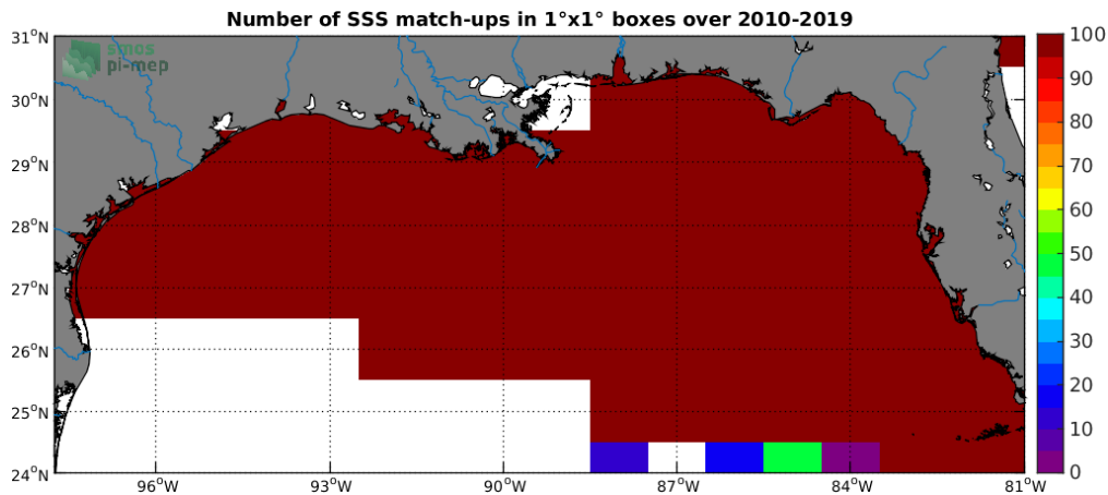
Figure 4: Number of SSS match-ups between TSG-SAMOS SSS and the SMOS-L3-CATDS-CECOS-LOCEAN-V4-18DAYS-25KM SSS product for the Mississippi river plume Pi-MEP region over 1°x1° boxes and for the full satellite product period.
