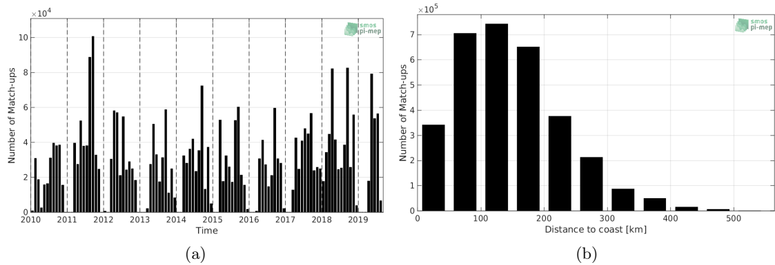
Figure 1: Number of match-ups between TSG-SAMOS and SMOS-L3-CATDS-CECOS-LOCEAN-V4-18DAYS-25KM SSS as a function of time (a) and as function of the distance to coast (b) over the Mississippi river plume Pi-MEP region and for the full satellite product period.
