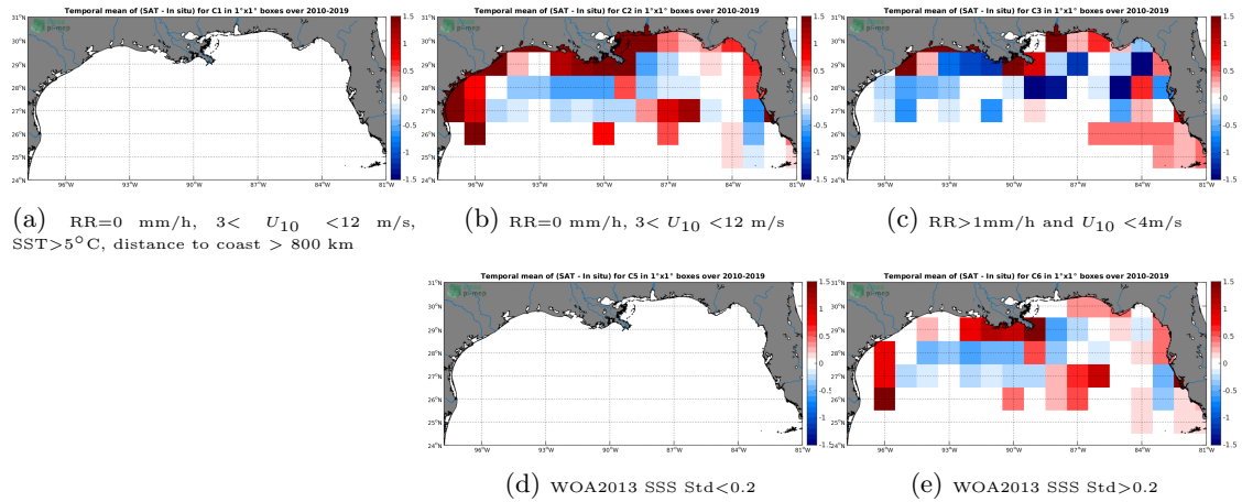
Figure 12: Temporal mean gridded over spatial boxes of size 1^\circ \times 1^\circ of \Delta SSS (SMOS-L3-CATDS-CECOS-LOCEAN-V4-18DAYS-25KM - TSG-SAMOS) for 5 different subdatasets corresponding to:RR=0 mm/h, 3 < U_{10} < 12 m/s, SST >5^\circ C, distance to coast > 800 km (a), RR=0 mm/h, 3 < U_{10} < 12 m/s (b), RR >1 mm/h and U_{10} < 4 m/s (c), WOA2013 SSS Std <0.2 (d), WOA2013 SSS Std >0.2 (e).
