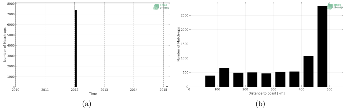
Figure 1: Number of match-ups between TSG (GOSUD-Sailing-ship) and SMOS SSS L3 v4 - 18 Days (CATDS-CECOS-LOCEAN) SSS as a function of time (a) and as function of the distance to coast (b) over the Mississippi river plume Pi-MEP region and for the full satellite product period.
