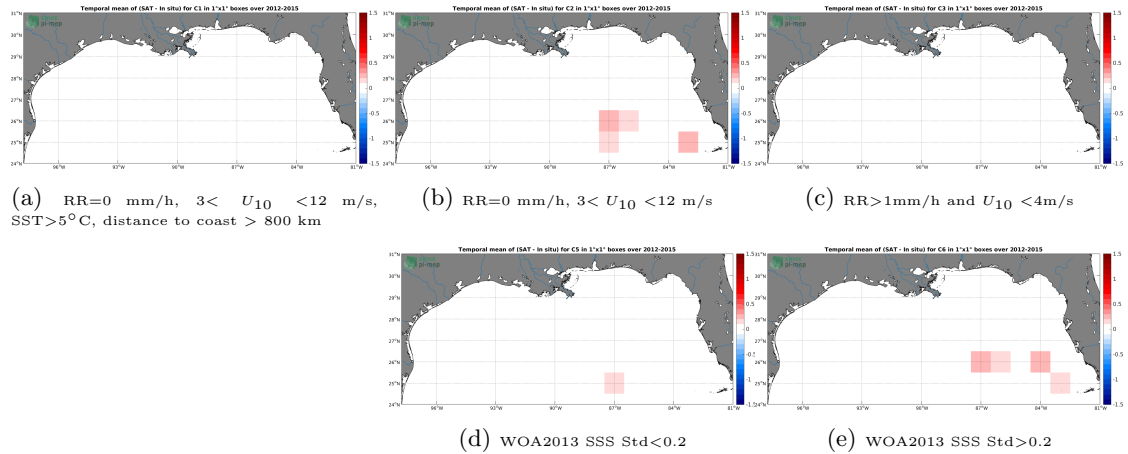
Figure 12: Temporal mean gridded over spatial boxes of size 1^\circ \times 1^\circ of \Delta SSS (SMOS SSS L3 v4 - 18 Days (CATDS-CECOS-LOCEAN) - TSG (GOSUD-Sailing-ship)) for 5 different subdatasets corresponding to: RR=0 mm/h, 3 < U_{10} < 12 m/s, SST > 5^\circ\text{C} , distance to coast > 800 km (a), RR=0 mm/h, 3 < U_{10} < 12 m/s (b), RR > 1 mm/h and U_{10} < 4 m/s (c), WOA2013 SSS Std < 0.2 (d), WOA2013 SSS Std > 0.2 (e).
