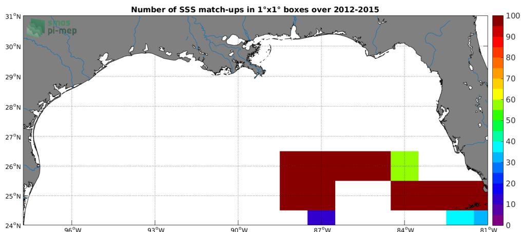
Figure 4: Number of SSS match-ups between TSG (GOSUD-Sailing-ship) SSS and the SMOS SSS L3 v4 - 18 Days (CATDS-CECOS-LOCEAN) SSS product for the Mississippi river plume Pi-MEP region over 1^\circ \times 1^\circ boxes and for the full satellite product period.
