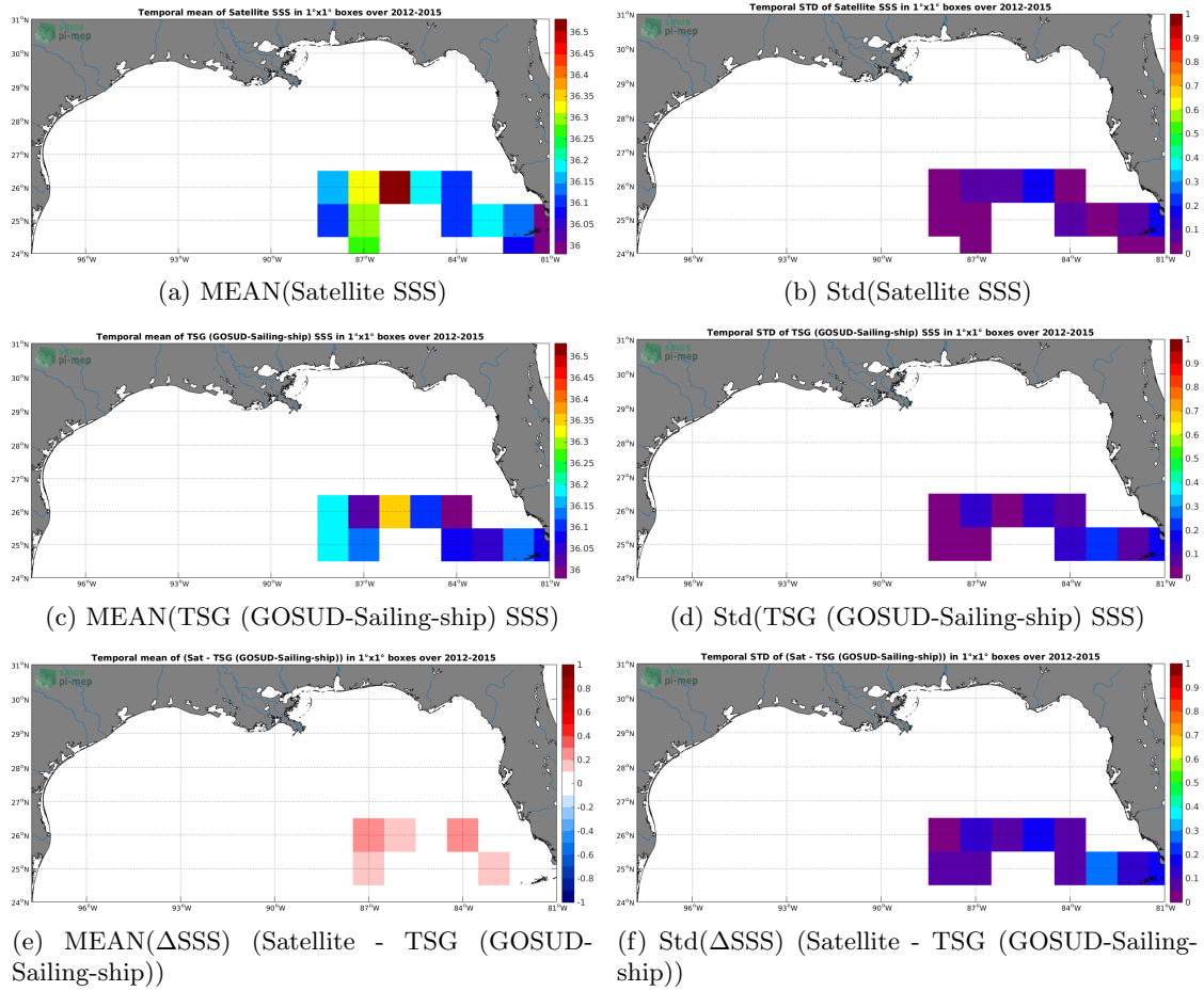
Figure 6: Temporal mean (left) and Std (right) of SSS from SMOS SSS L3 v4 - 18 Days (CATDS-CECOS-LOCEAN) (top), TSG (GOSUD-Sailing-ship) (middle), and of \Delta SSS (Satellite - TSG (GOSUD-Sailing-ship)). Only match-up pairs are used to generate these maps.
