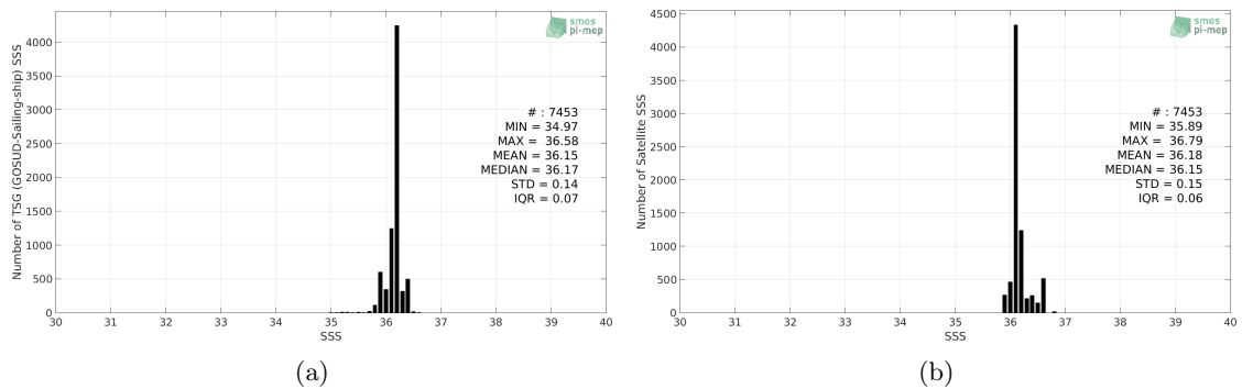
Figure 2: Histograms of SSS from TSG (GOSUD-Sailing-ship) (a) and SMOS SSS L3 v4 - 18 Days (CATDS-CECOS-LOCEAN) (b) considering all match-up pairs per bins of 0.1 over the Mississippi river plume Pi-MEP region and for the full satellite product period.
