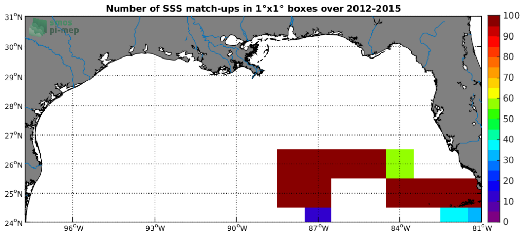
Figure 4: Number of SSS match-ups between TSG-GOSUD-Sailing-ship SSS and the SMOS-L3-CATDS-CECOS-LOCEAN-V4-18DAYS-25KM SSS product for the Mississippi river plume Pi-MEP region over 1^\circ \times 1^\circ boxes and for the full satellite product period.
