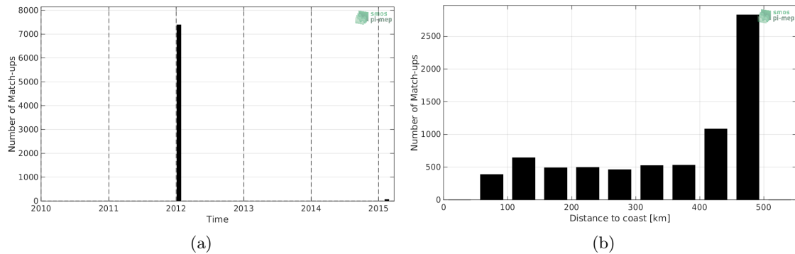
Figure 1: Number of match-ups between TSG-GOSUD-Sailing-ship and SMOS-L3-CATDS-CECOS-LOCEAN-V4-18DAYS-25KM SSS as a function of time (a) and as function of the distance to coast (b) over the Mississippi river plume Pi-MEP region and for the full satellite product period.
