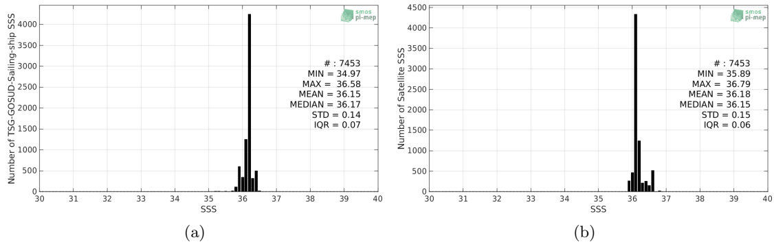
Figure 2: Histograms of SSS from TSG-GOSUD-Sailing-ship (a) and SMOS-L3-CATDS-CECOS-LOCEAN-V4-18DAYS-25KM (b) considering all match-up pairs per bins of 0.1 over the Mississippi river plume Pi-MEP region and for the full satellite product period.
