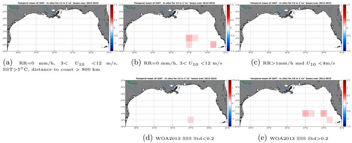
Figure 12: Temporal mean gridded over spatial boxes of size 1^\circ \times 1^\circ of \Delta SSS (SMOS-L3-CATDS-CECOS-LOCEAN-V4-18DAYS-25KM - TSG-GOSUD-Sailing-ship) for 5 different subdatasets corresponding to: RR=0 mm/h, 3 < U_{10} < 12 m/s, SST > 5°C, distance to coast > 800 km (a), RR=0 mm/h, 3 < U_{10} < 12 m/s (b), RR > 1mm/h and U_{10} < 4 m/s (c), WOA2013 SSS Std < 0.2 (d), WOA2013 SSS Std > 0.2 (e).
