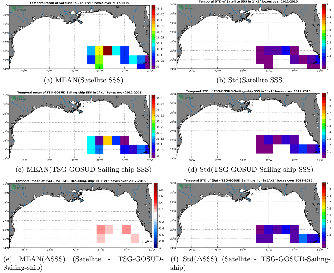
Figure 6: Temporal mean (left) and Std (right) of SSS from SMOS-L3-CATDS-CECOS-LOCEAN-V4-18DAYS-25KM (top), TSG-GOSUD-Sailing-ship (middle), and of \Delta SSS (Satellite - TSG-GOSUD-Sailing-ship). Only match-up pairs are used to generate these maps.
