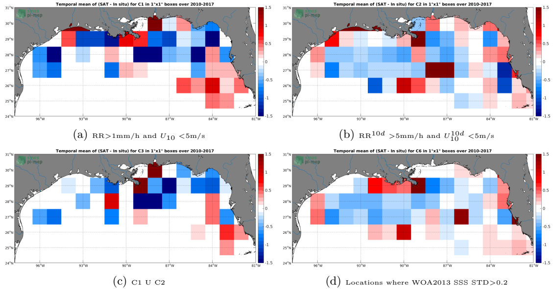
Figure 12: Temporal mean gridded over spatial boxes of size 1^\circ \times 1^\circ of \Delta SSS (SMOS-L3-CATDS-CECOS-LOCEAN-V3-9DAYS-25KM - TSG-SAMOS) for 4 different subdatasets corresponding to: RR > 1mm/h and U_{10} < 5\text{m/s} (a), RR^{10d} > 5\text{mm/h} and U_{10}^{10d} < 5\text{m/s} (b), C1 U C2 (c), Locations where WOA2013 SSS STD > 0.2 (d).
