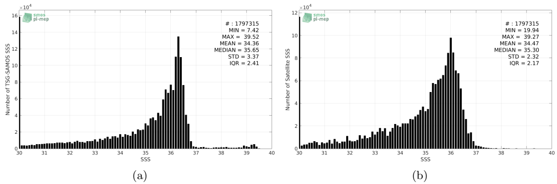
Figure 2: Histograms of SSS from TSG-SAMOS (a) and SMOS-L3-CATDS-CECOS-LOCEAN-V3-9DAYS-25KM (b) considering all match-up pairs per bins of 0.1 over the Mississippi river plume Pi-MEP region and for the full satellite product period.
