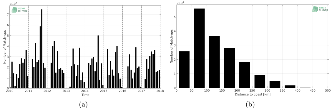
Figure 1: Number of match-ups between TSG-SAMOS and SMOS-L3-CATDS-CECOS-LOCEAN-V3-9DAYS-25KM SSS as a function of time (a) and as function of the distance to coast (b) over the Mississippi river plume Pi-MEP region and for the full satellite product period.
