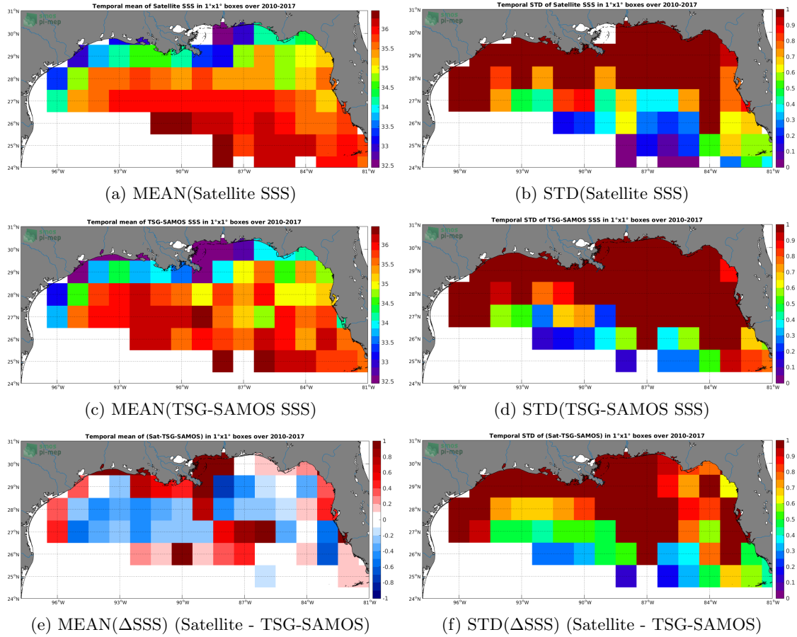
Figure 6: Temporal mean (left) and STD (right) of SSS from SMOS-L3-CATDS-CECOS-LOCEAN-V3-9DAYS-25KM (top), TSG-SAMOS (middle), and of \Delta SSS (Satellite - TSG-SAMOS). Only match-up pairs are used to generate these maps.
