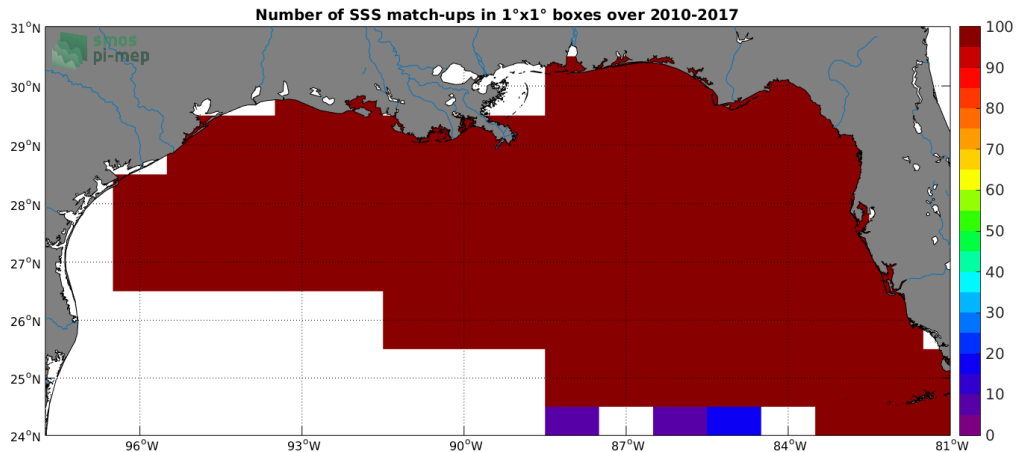
Figure 4: Number of SSS match-ups between TSG-SAMOS SSS and the SMOS-L3-CATDS-CECOS-LOCEAN-V3-9DAYS-25KM SSS product for the Mississippi river plume Pi-MEP region over 1^\circ \times 1^\circ boxes and for the full satellite product period.
