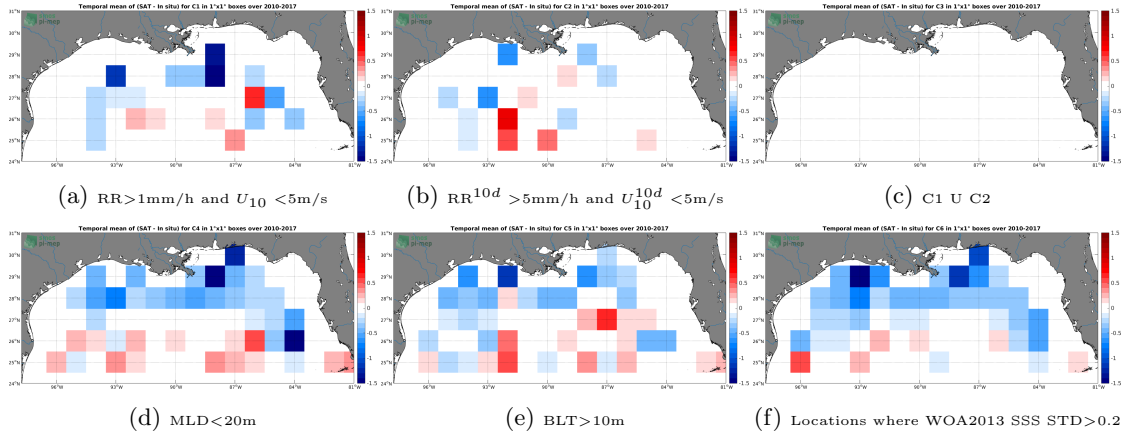
Figure 12: Temporal mean gridded over spatial boxes of size 1^\circ \times 1^\circ of \Delta\text{SSS} (SMOS-L3-CATDS-CECOS-LOCEAN-V3-9DAYS-25KM - Argo) for 6 different subdatasets corresponding to: \text{RR} > 1\text{mm/h} and U_{10} < 5\text{m/s} (a), \text{RR}^{10d} > 5\text{mm/h} and U_{10}^{10d} < 5\text{m/s} (b), C1 U C2 (c), \text{MLD} < 20\text{m} (d), \text{BLT} > 10\text{m} (e), Locations where WOA2013 SSS \text{STD} > 0.2 (f).
