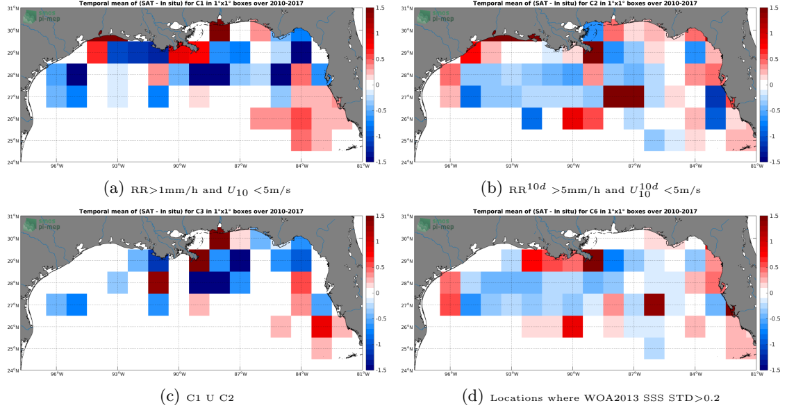
Figure 12: Temporal mean gridded over spatial boxes of size 1^\circ \times 1^\circ of \Delta SSS (SMOS-L3-CATDS-CECOS-LOCEAN-V3-18DAYS-25KM - TSG-SAMOS) for 4 different subdatasets corresponding to: RR > 1\text{mm/h} and U_{10} < 5\text{m/s} (a), RR^{10d} > 5\text{mm/h} and U_{10}^{10d} < 5\text{m/s} (b), C1 U C2 (c), Locations where WOA2013 SSS STD > 0.2 (d).
