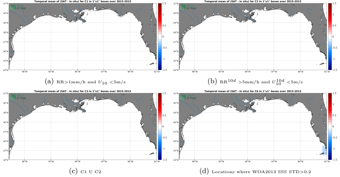
Figure 12: Temporal mean gridded over spatial boxes of size 1^\circ \times 1^\circ of \Delta SSS (SMOS-L3-CATDS-CECOS-LOCEAN-V3-18DAYS-25KM - TSG-GOSUD-Sailing-ship) for 4 different subdatasets corresponding to: RR > 1\text{mm/h} and U_{10} < 5\text{m/s} (a), RR^{10d} > 5\text{mm/h} and U_{10}^{10d} < 5\text{m/s} (b), C1 \cup C2 (c), Locations where WOA2013 SSS STD > 0.2 (d).
