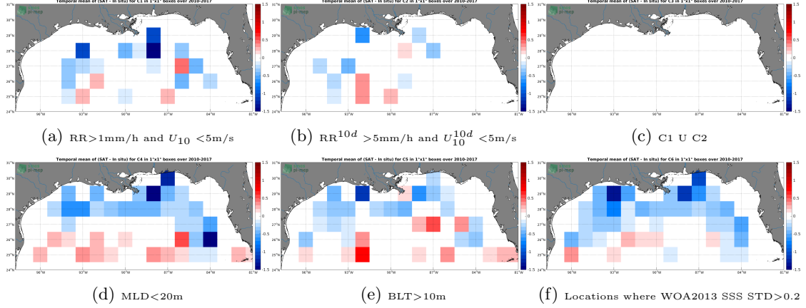
Figure 12: Temporal mean gridded over spatial boxes of size 1^\circ \times 1^\circ of \Delta SSS (SMOS-L3-CATDS-CECOS-LOCEAN-V3-18DAYS-25KM - Argo) for 6 different subdatasets corresponding to: RR>1\text{mm/h} and U_{10}<5\text{m/s} (a), RR^{10d}>5\text{mm/h} and U_{10}^{10d}<5\text{m/s} (b), C1 U C2 (c), MLD<20\text{m} (d), BLT>10\text{m} (e), Locations where WOA2013 SSS STD>0.2 (f).
