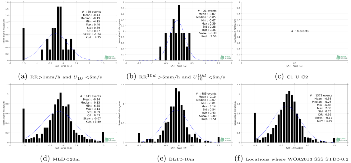
Figure 13: Normalized histogram of \Delta SSS (SMOS-L3-CATDS-CECOS-LOCEAN-V3-18DAYS-25KM - Argo) for 6 different subdatasets corresponding to: RR>1\text{mm/h} and U_{10}<5\text{m/s} (a), RR^{10d}>5\text{mm/h} and U_{10}^{10d}<5\text{m/s} (b), C1 U C2 (c), MLD<20\text{m} (d), BLT>10\text{m} (e), Locations where WOA2013 SSS STD>0.2 (f).
