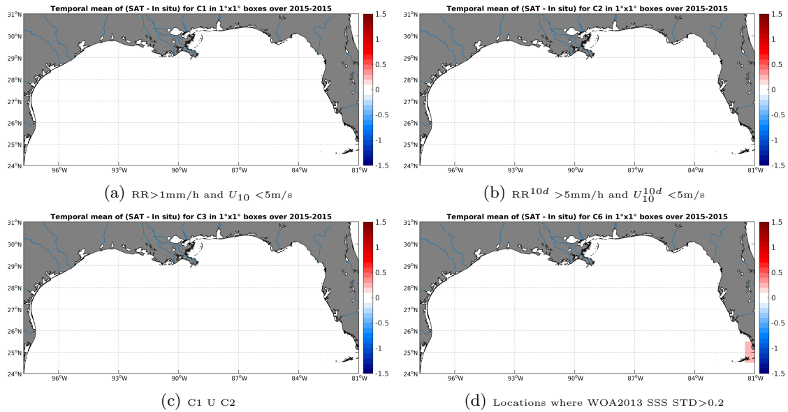
Figure 12: Temporal mean gridded over spatial boxes of size 1^\circ \times 1^\circ of \Delta SSS (SMOS-L3-CATDS-CECOS-LOCEAN-V2-9DAYS-25KM - TSG-GOSUD-Sailing-ship) for 4 different subdatasets corresponding to: RR > 1\text{mm/h} and U_{10} < 5\text{m/s} (a), RR^{10d} > 5\text{mm/h} and U_{10}^{10d} < 5\text{m/s} (b), C1 U C2 (c), Locations where WOA2013 SSS STD > 0.2 (d).
