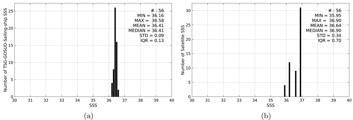
Figure 2: Histograms of SSS from TSG-GOSUD-Sailing-ship (a) and SMOS-L3-CATDS-CECOS-LOCEAN-V2-9DAYS-25KM (b) considering all match-up pairs per bins of 0.1 over the Mississippi river plume Pi-MEP region and for the full satellite product period.
