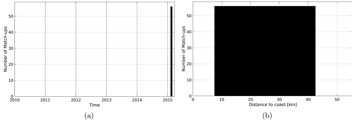
Figure 1: Number of match-ups between TSG-GOSUD-Sailing-ship and SMOS-L3-CATDS-CECOS-LOCEAN-V2-9DAYS-25KM SSS as a function of time (a) and as function of the distance to coast (b) over the Mississippi river plume Pi-MEP region and for the full satellite product period.
