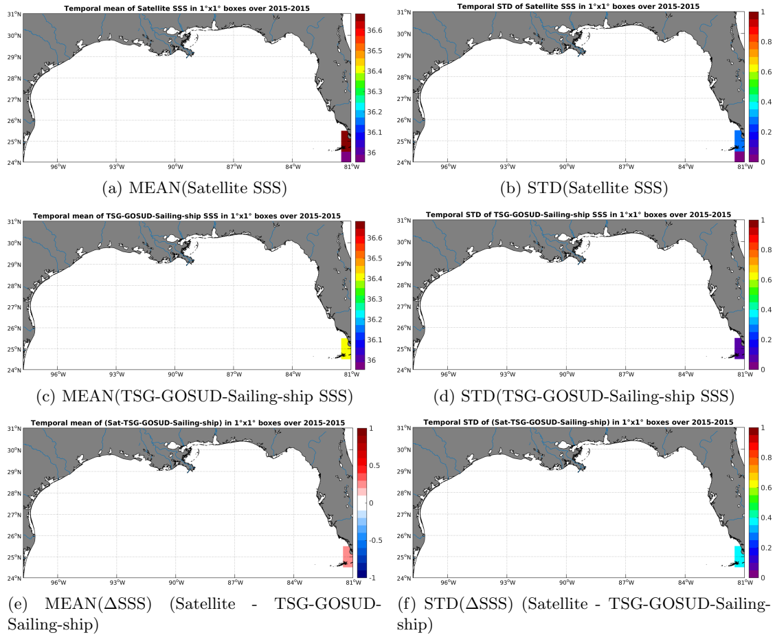
Figure 6: Temporal mean (left) and STD (right) of SSS from SMOS-L3-CATDS-CECOS-LOCEAN-V2-9DAYS-25KM (top), TSG-GOSUD-Sailing-ship (middle), and of \Delta SSS (Satellite - TSG-GOSUD-Sailing-ship). Only match-up pairs are used to generate these maps.
