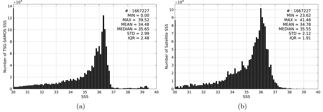
Figure 2: Histograms of SSS from TSG-SAMOS (a) and SMOS-L3-CATDS-CECOS-LOCEAN-V2-18DAYS-25KM (b) considering all match-up pairs per bins of 0.1 over the Mississippi river plume Pi-MEP region and for the full satellite product period.
