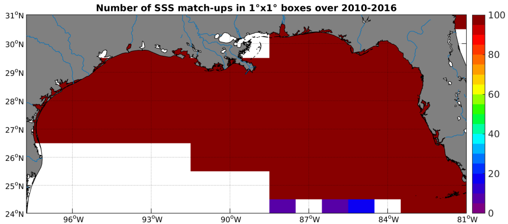
Figure 4: Number of SSS match-ups between TSG-SAMOS SSS and the SMOS-L3-CATDS-CECOS-LOCEAN-V2-18DAYS-25KM SSS product for the Mississippi river plume Pi-MEP region over 1^\circ \times 1^\circ boxes and for the full satellite product period.
