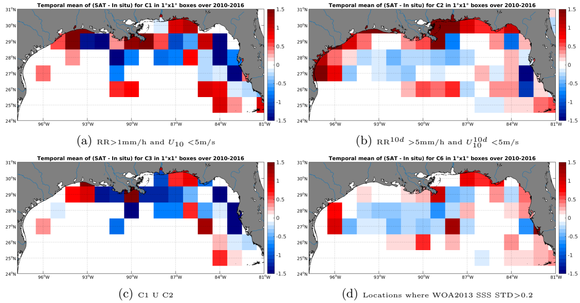
Figure 12: Temporal mean gridded over spatial boxes of size 1^\circ \times 1^\circ of \Delta SSS (SMOS-L3-CATDS-CECOS-LOCEAN-V2-18DAYS-25KM - TSG-SAMOS) for 4 different subdatasets corresponding to: RR > 1mm/h and U_{10} < 5 m/s (a), RR 10d > 5mm/h and U_{10}^{10d} < 5 m/s (b), C1 U C2 (c), Locations where WOA2013 SSS STD > 0.2 (d).
