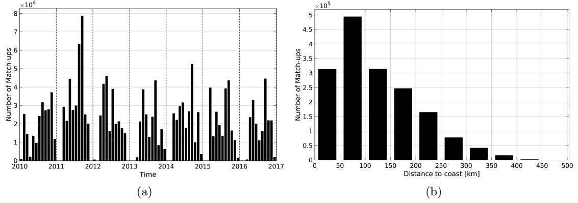
Figure 1: Number of match-ups between TSG-SAMOS and SMOS-L3-CATDS-CECOS-LOCEAN-V2-18DAYS-25KM SSS as a function of time (a) and as function of the distance to coast (b) over the Mississippi river plume Pi-MEP region and for the full satellite product period.
