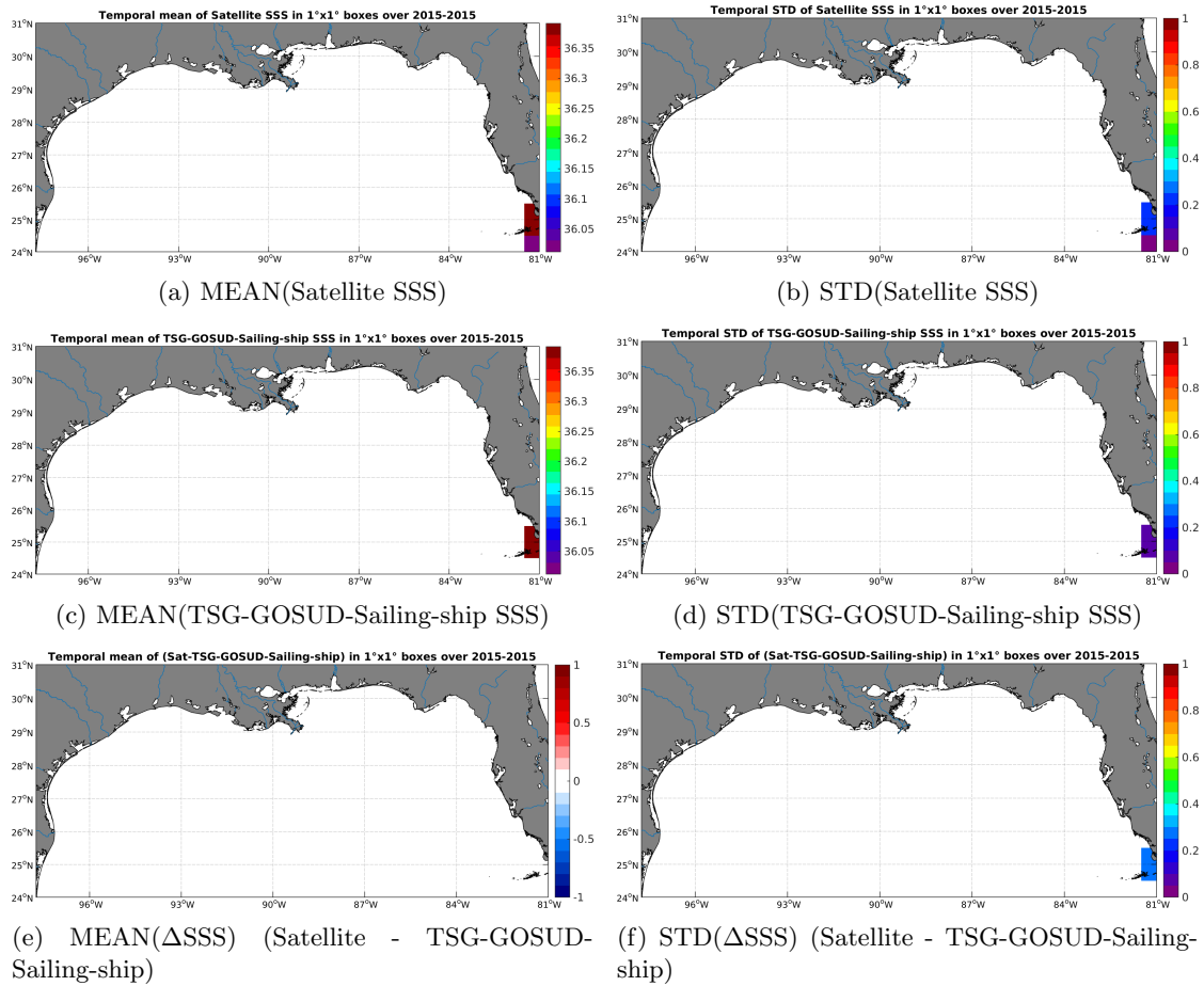
Figure 6: Temporal mean (left) and STD (right) of SSS from SMOS-L3-CATDS-CECOS-LOCEAN-V2-18DAYS-25KM (top), TSG-GOSUD-Sailing-ship (middle), and of \Delta SSS (Satellite - TSG-GOSUD-Sailing-ship). Only match-up pairs are used to generate these maps.
