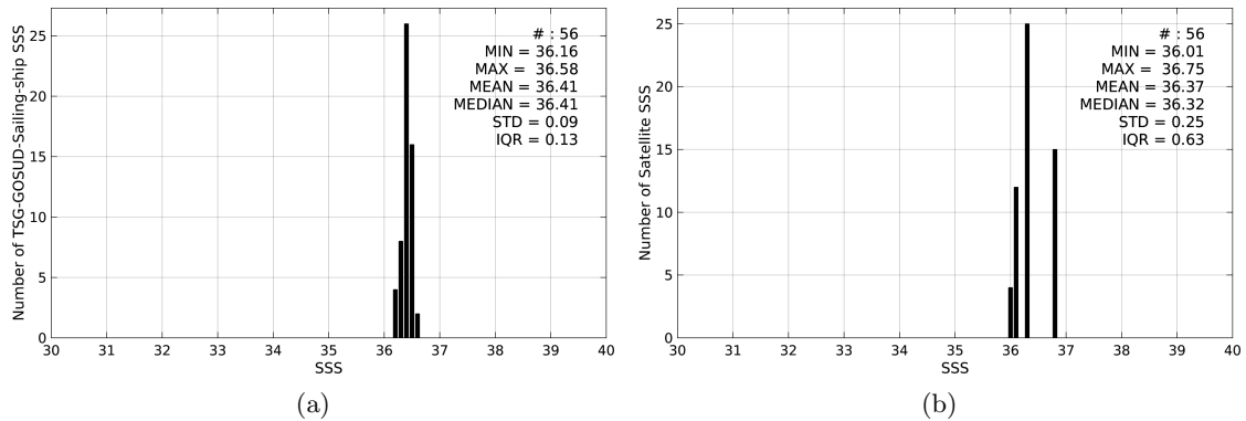
Figure 2: Histograms of SSS from TSG-GOSUD-Sailing-ship (a) and SMOS-L3-CATDS-CECOS-LOCEAN-V2-18DAYS-25KM (b) considering all match-up pairs per bins of 0.1 over the Mississippi river plume Pi-MEP region and for the full satellite product period.
