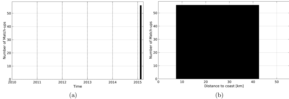
Figure 1: Number of match-ups between TSG-GOSUD-Sailing-ship and SMOS-L3-CATDS-CECOS-LOCEAN-V2-18DAYS-25KM SSS as a function of time (a) and as function of the distance to coast (b) over the Mississippi river plume Pi-MEP region and for the full satellite product period.
