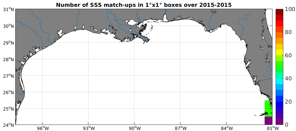
Figure 4: Number of SSS match-ups between TSG-GOSUD-Sailing-ship SSS and the SMOS-L3-CATDS-CECOS-LOCEAN-V2-18DAYS-25KM SSS product for the Mississippi river plume Pi-MEP region over 1^\circ \times 1^\circ boxes and for the full satellite product period.
