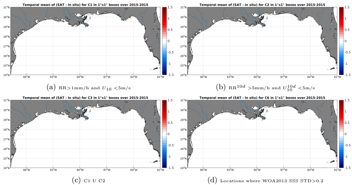
Figure 12: Temporal mean gridded over spatial boxes of size 1^\circ \times 1^\circ of \Delta SSS (SMOS-L3-CATDS-CECOS-LOCEAN-V2-18DAYS-25KM - TSG-GOSUD-Sailing-ship) for 4 different subdatasets corresponding to:RR >1 mm/h and U_{10} < 5 m/s (a), RR^{10d} > 5 mm/h and U_{10}^{10d} < 5 m/s (b), C1 U C2 (c),Locations where WOA2013 SSS STD >0.2 (d).
