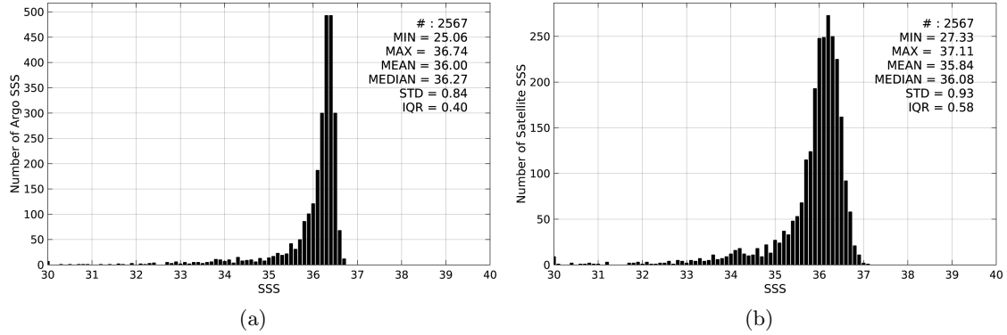
Figure 2: Histograms of SSS from Argo (a) and SMOS-L3-CATDS-CECOS-LOCEAN-V2-18DAYS-25KM (b) considering all match-up pairs per bins of 0.1 over the Mississippi river plume Pi-MEP region and for the full satellite product period.
