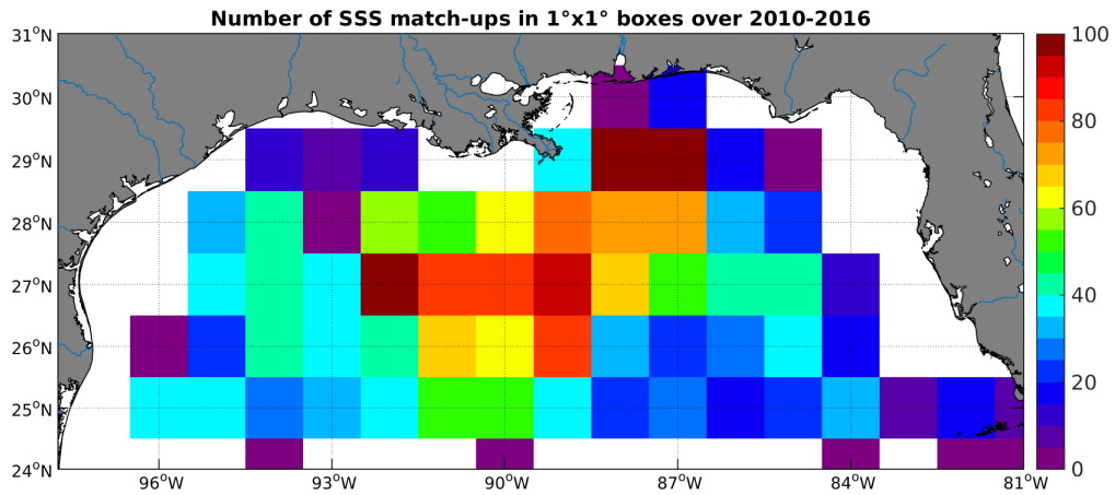
Figure 4: Number of SSS match-ups between Argo SSS and the SMOS-L3-CATDS-CECOS-LOCEAN-V2-18DAYS-25KM SSS product for the Mississippi river plume Pi-MEP region over 1^\circ \times 1^\circ boxes and for the full satellite product period.
