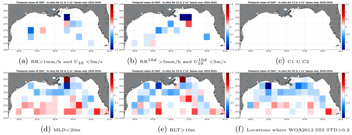
Figure 12: Temporal mean gridded over spatial boxes of size 1^\circ \times 1^\circ of \Delta SSS (SMOS-L3-CATDS-CECOS-LOCEAN-V2-18DAYS-25KM - Argo) for 6 different subdatasets corresponding to: RR > 1\text{mm/h} and U_{10} < 5\text{m/s} (a), RR^{10d} > 5\text{mm/h} and U_{10}^{10d} < 5\text{m/s} (b), C1 U C2 (c), MLD < 20\text{m} (d), BLT > 10\text{m} (e), Locations where WOA2013 SSS STD > 0.2 (f).
