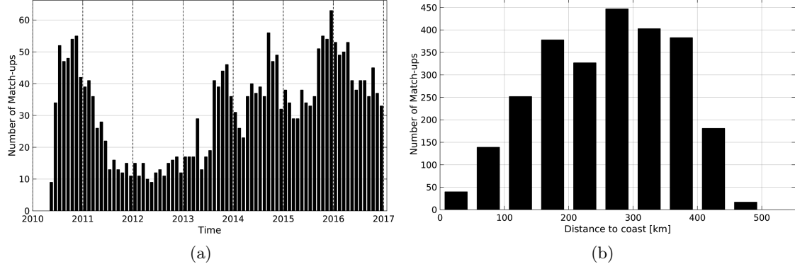
Figure 1: Number of match-ups between Argo and SMOS-L3-CATDS-CECOS-LOCEAN-V2-18DAYS-25KM SSS as a function of time (a) and as function of the distance to coast (b) over the Mississippi river plume Pi-MEP region and for the full satellite product period.
