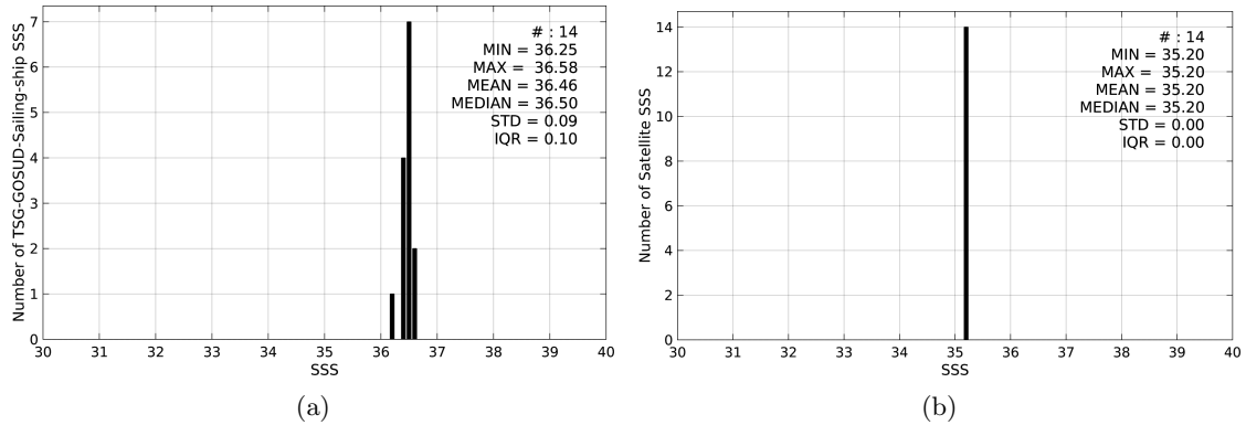
Figure 2: Histograms of SSS from TSG-GOSUD-Sailing-ship (a) and SMOS-L3-CATDS-IFREMER-CECOS-V2-MONTHLY-0.25DEG (b) considering all match-up pairs per bins of 0.1 over the Mississippi river plume Pi-MEP region and for the full satellite product period.
