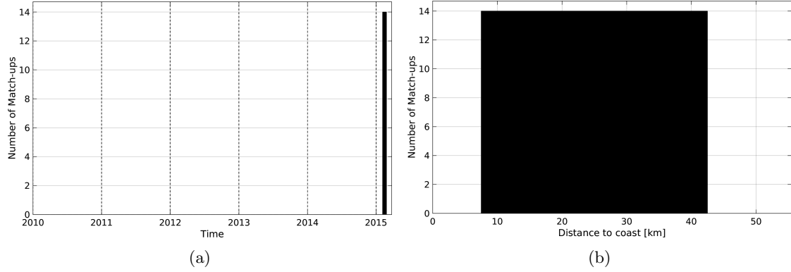
Figure 1: Number of match-ups between TSG-GOSUD-Sailing-ship and SMOS-L3-CATDS-IFREMER-CECOS-V2-MONTHLY-0.25DEG SSS as a function of time (a) and as function of the distance to coast (b) over the Mississippi river plume Pi-MEP region and for the full satellite product period.
