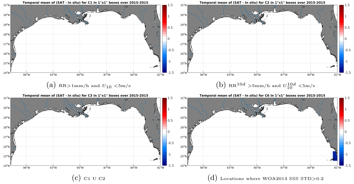
Figure 12: Temporal mean gridded over spatial boxes of size 1^\circ \times 1^\circ of \Delta SSS (SMOS-L3-CATDS-IFREMER-CECOS-V2-MONTHLY-0.25DEG - TSG-GOSUD-Sailing-ship) for 4 different sub-datasets corresponding to: RR > 1\text{mm/h} and U_{10} < 5\text{m/s} (a), RR^{10d} > 5\text{mm/h} and U_{10}^{10d} < 5\text{m/s} (b), C1 U C2 (c), Locations where WOA2013 SSS STD > 0.2 (d).
