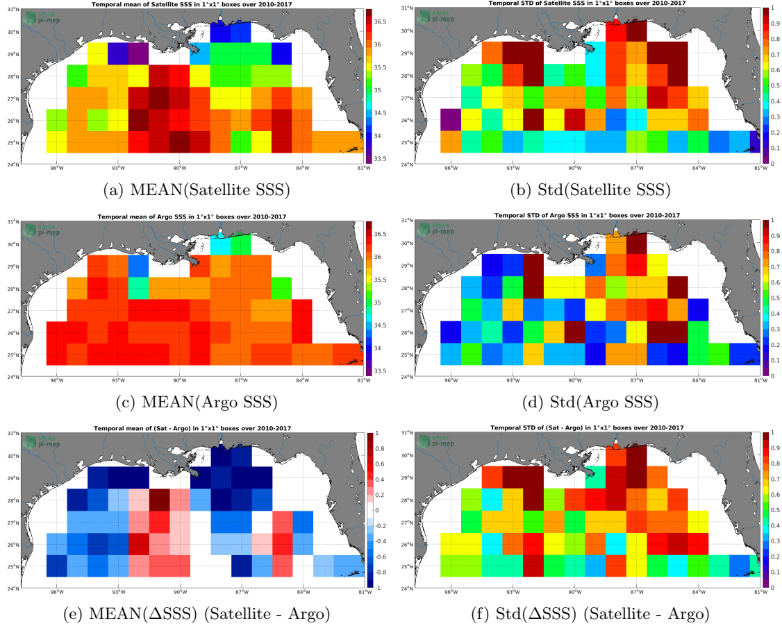
Figure 6: Temporal mean (left) and Std (right) of SSS from SMOS SSS L3 v2 - Monthly - 0.25 Deg (CATDS-CECOS-IFREMER) (top), Argo (middle), and of \Delta SSS (Satellite - Argo). Only match-up pairs are used to generate these maps.
