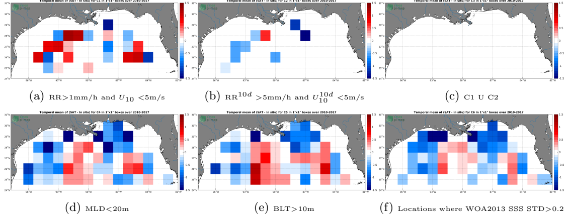
Figure 12: Temporal mean gridded over spatial boxes of size 1^\circ \times 1^\circ of \Delta\text{SSS} (SMOS-L3-CATDS-IFREMER-CECOS-V2-MONTHLY-0.25DEG - Argo) for 6 different subdatasets corresponding to: \text{RR} > 1\text{mm/h} and U_{10} < 5\text{m/s} (a), \text{RR}^{10d} > 5\text{mm/h} and U_{10}^{10d} < 5\text{m/s} (b), C1 U C2 (c), \text{MLD} < 20\text{m} (d), \text{BLT} > 10\text{m} (e), Locations where WOA2013 SSS STD > 0.2 (f).
