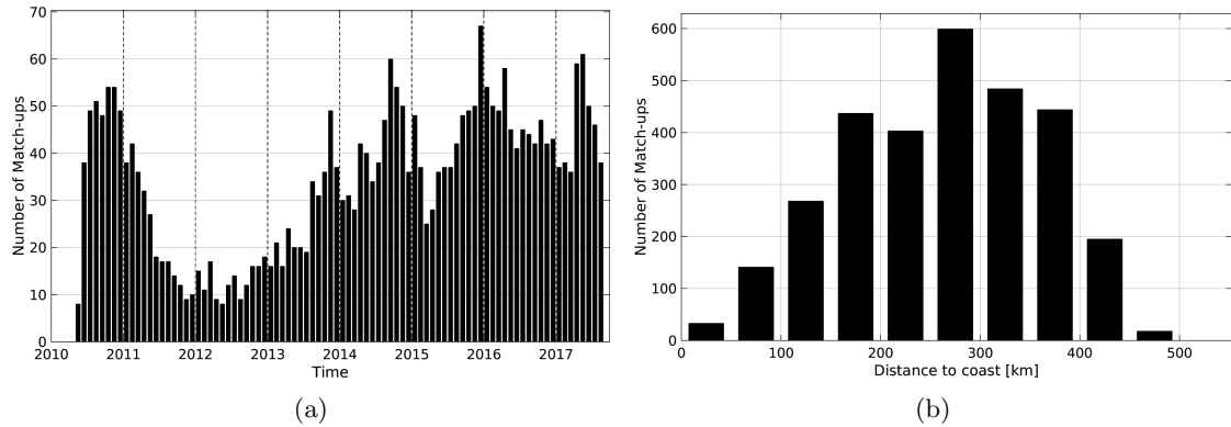
Figure 1: Number of match-ups between Argo and SMOS-L3-CATDS-IFREMER-CECOS-V2-MONTHLY-0.25DEG SSS as a function of time (a) and as function of the distance to coast (b) over the Mississippi river plume Pi-MEP region and for the full satellite product period.
