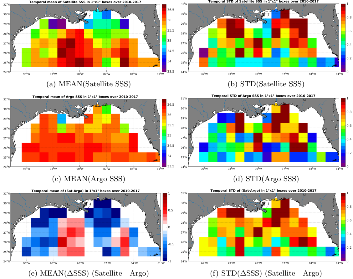
Figure 6: Temporal mean (left) and STD (right) of SSS from SMOS-L3-CATDS-IFREMER-CECOS-V2-MONTHLY-0.25DEG (top), Argo (middle), and of \Delta\text{SSS} (Satellite - Argo). Only match-up pairs are used to generate these maps.
