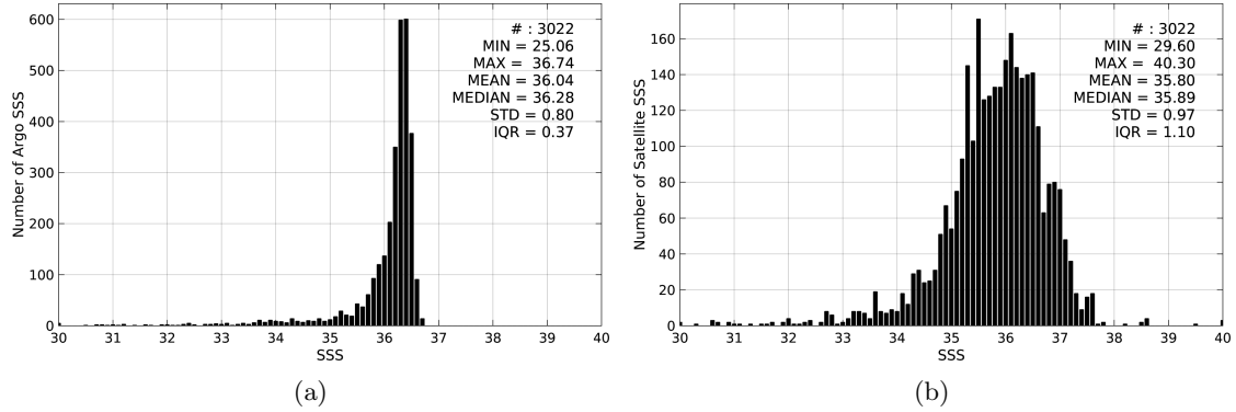
Figure 2: Histograms of SSS from Argo (a) and SMOS-L3-CATDS-IFREMER-CECOS-V2-MONTHLY-0.25DEG (b) considering all match-up pairs per bins of 0.1 over the Mississippi river plume Pi-MEP region and for the full satellite product period.
