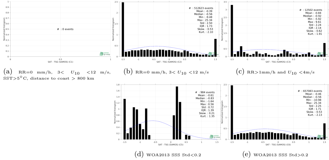
Figure 13: Normalized histogram of \Delta SSS (SMOS SSS L3 v2 - Daily - 0.5 Deg (CATDS-CECOS-IFREMER) - TSG (SAMOS)) for 5 different subdatasets corresponding to: RR=0 mm/h, 3 < U_{10} < 12 m/s, SST > 5°C, distance to coast > 800 km (a), RR=0 mm/h, 3 < U_{10} < 12 m/s (b), RR > 1mm/h and U_{10} < 4 m/s (c), WOA2013 SSS Std < 0.2 (d), WOA2013 SSS Std > 0.2 (e).
