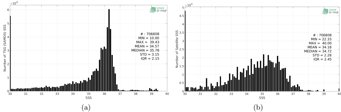
Figure 2: Histograms of SSS from TSG (SAMOS) (a) and SMOS SSS L3 v2 - Daily - 0.5 Deg (CATDS-CECOS-IFREMER) (b) considering all match-up pairs per bins of 0.1 over the Mississippi river plume Pi-MEP region and for the full satellite product period.
