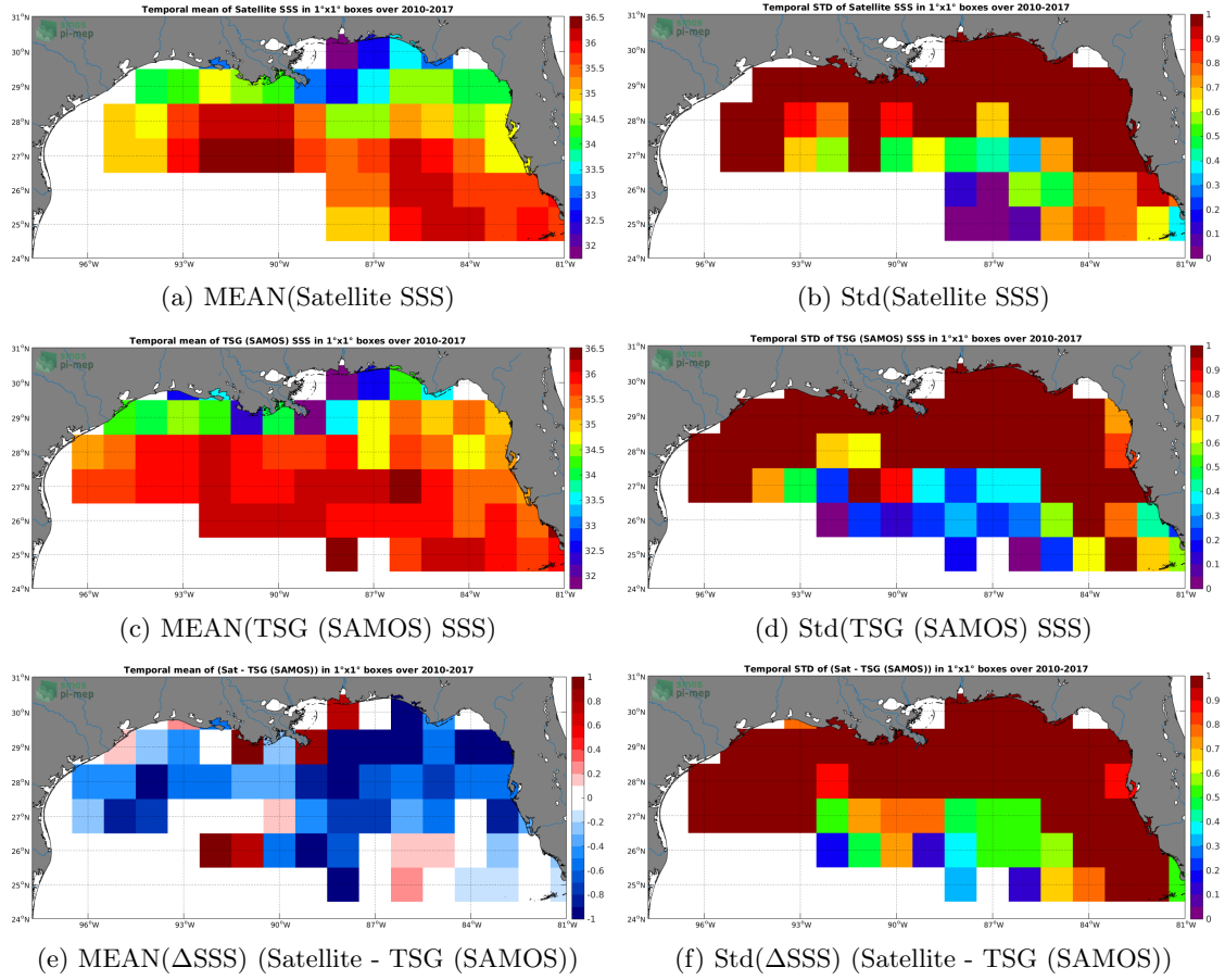
Figure 6: Temporal mean (left) and Std (right) of SSS from SMOS SSS L3 v2 - Daily - 0.5 Deg (CATDS-CECOS-IFREMER) (top), TSG (SAMOS) (middle), and of \Delta SSS (Satellite - TSG (SAMOS)). Only match-up pairs are used to generate these maps.
