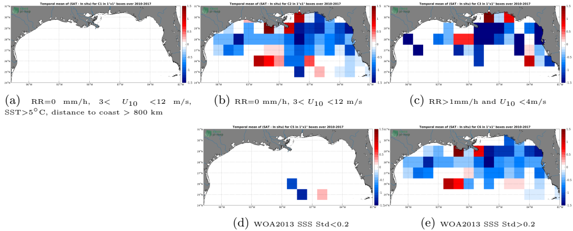
Figure 12: Temporal mean gridded over spatial boxes of size 1^{\circ}\times 1^{\circ} of \Delta\text{SSS} (SMOS SSS L3 v2 - Daily - 0.5 Deg (CATDS-CECOS-IFREMER) - TSG (SAMOS)) for 5 different subdatasets corresponding to:RR=0 mm/h, 3 < U_{10} < 12 m/s, SST >5^{\circ}\text{C} , distance to coast > 800 km (a), RR=0 mm/h, 3 < U_{10} < 12 m/s (b), RR >1 mm/h and U_{10} < 4 m/s (c), WOA2013 SSS Std <0.2 (d), WOA2013 SSS Std >0.2 (e).
