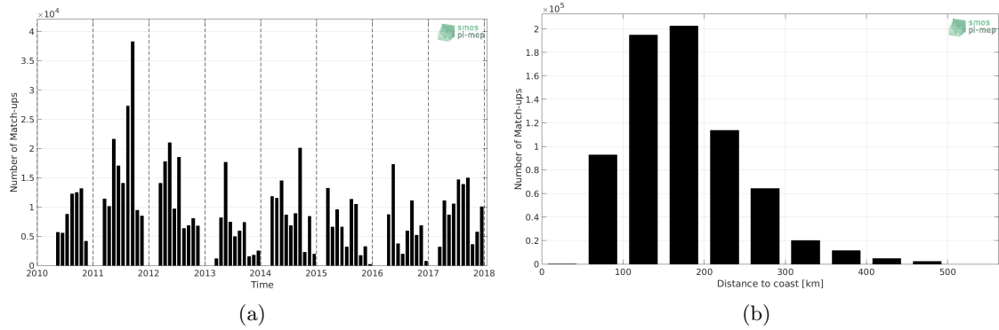
Figure 1: Number of match-ups between TSG (SAMOS) and SMOS SSS L3 v2 - Daily - 0.5 Deg (CATDS-CECOS-IFREMER) SSS as a function of time (a) and as function of the distance to coast (b) over the Mississippi river plume Pi-MEP region and for the full satellite product period.
