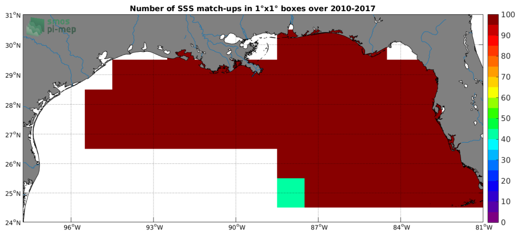
Figure 4: Number of SSS match-ups between TSG (SAMOS) SSS and the SMOS SSS L3 v2 - Daily - 0.5 Deg (CATDS-CECOS-IFREMER) SSS product for the Mississippi river plume Pi-MEP region over 1^\circ \times 1^\circ boxes and for the full satellite product period.
