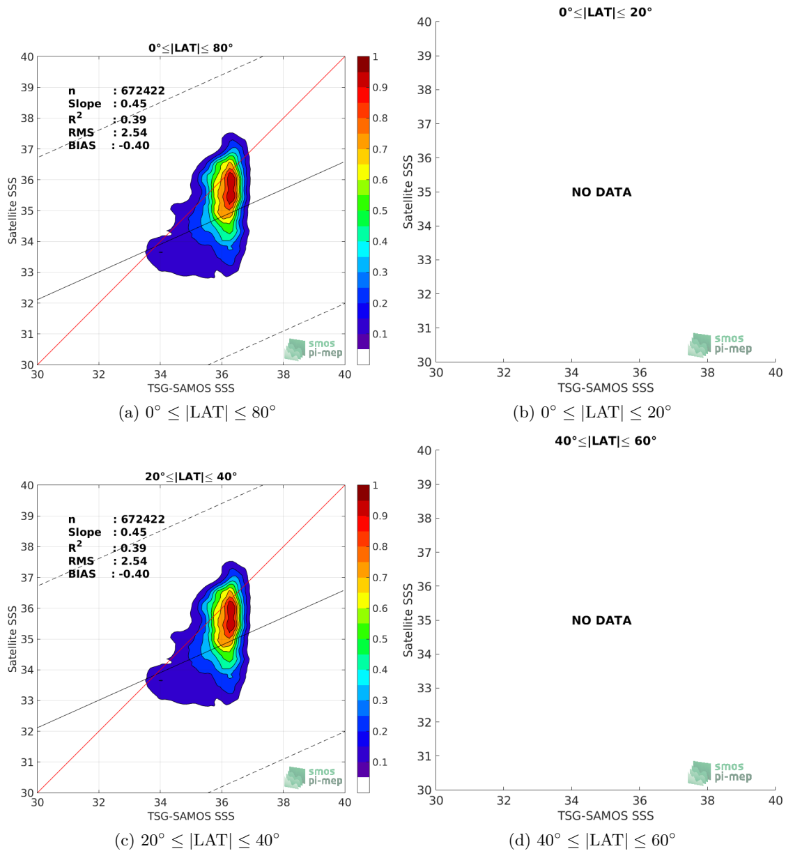
Figure 9: Contour maps of the concentration of SMOS L3 v2 - Daily - 0.5 Deg (CATDS-CECOS-IFREMER) SSS (y-axis) versus TSG-SAMOS SSS (x-axis) at match-up pairs for different latitude bands. For each plot, the red line shows x=y . The black thin and dashed lines indicate a linear fit through the data cloud and the \pm 95\% confidence levels, respectively. The number match-up pairs n , the slope and R^2 coefficient of the linear fit, the root mean square (RMS) and the mean bias between satellite and in situ data are indicated for each latitude band in each plots.
