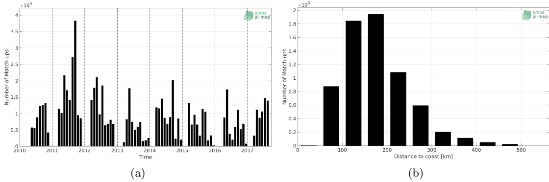
Figure 1: Number of match-ups between TSG-SAMOS and SMOS L3 v2 - Daily - 0.5 Deg (CATDS-CECOS-IFREMER) SSS as a function of time (a) and as function of the distance to coast (b) over the Mississippi river plume Pi-MEP region and for the full satellite product period.
