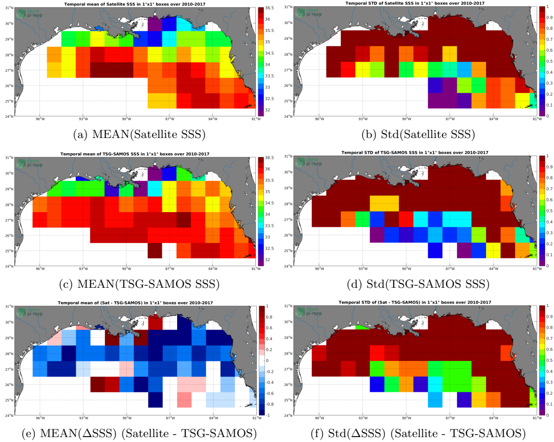
Figure 6: Temporal mean (left) and Std (right) of SSS from SMOS L3 v2 - Daily - 0.5 Deg (CATDS-CECOS-IFREMER) (top), TSG-SAMOS (middle), and of \Delta SSS (Satellite - TSG-SAMOS). Only match-up pairs are used to generate these maps.
