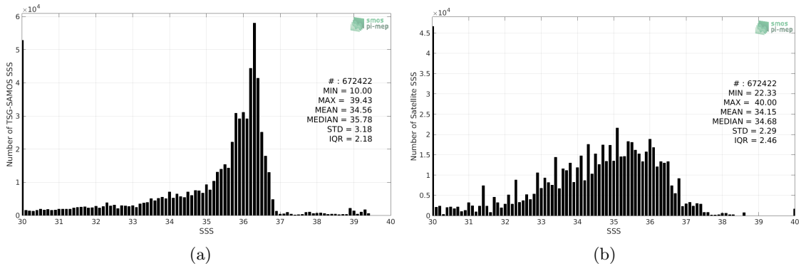
Figure 2: Histograms of SSS from TSG-SAMOS (a) and SMOS L3 v2 - Daily - 0.5 Deg (CATDS-CECOS-IFREMER) (b) considering all match-up pairs per bins of 0.1 over the Mississippi river plume Pi-MEP region and for the full satellite product period.
