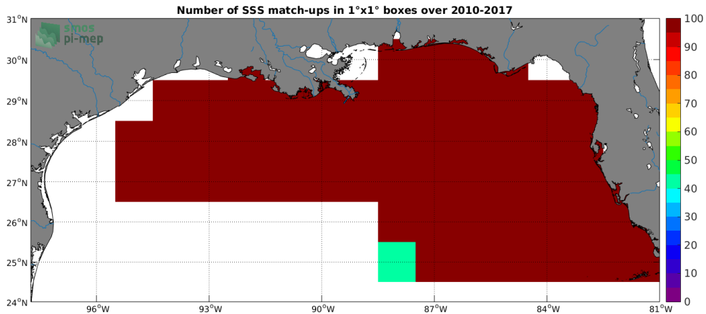
Figure 4: Number of SSS match-ups between TSG-SAMOS SSS and the SMOS L3 v2 - Daily - 0.5 Deg (CATDS-CECOS-IFREMER) SSS product for the Mississippi river plume Pi-MEP region over 1^\circ \times 1^\circ boxes and for the full satellite product period.
