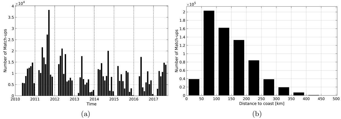
Figure 1: Number of match-ups between TSG-SAMOS and SMOS-L3-CATDS-CECOS-IFREMER-V2-1DAY-0.5DEG SSS as a function of time (a) and as function of the distance to coast (b) over the Mississippi river plume Pi-MEP region and for the full satellite product period.
