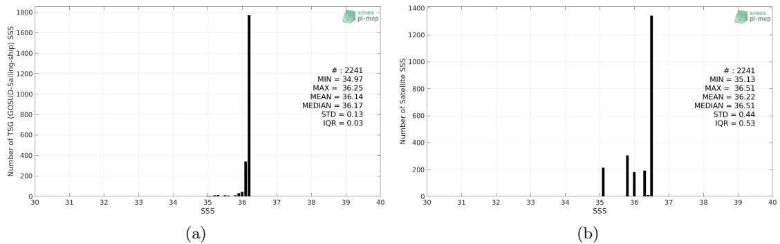
Figure 2: Histograms of SSS from TSG (GOSUD-Sailing-ship) (a) and SMOS SSS L3 v2 - Daily - 0.5 Deg (CATDS-CECOS-IFREMER) (b) considering all match-up pairs per bins of 0.1 over the Mississippi river plume Pi-MEP region and for the full satellite product period.
