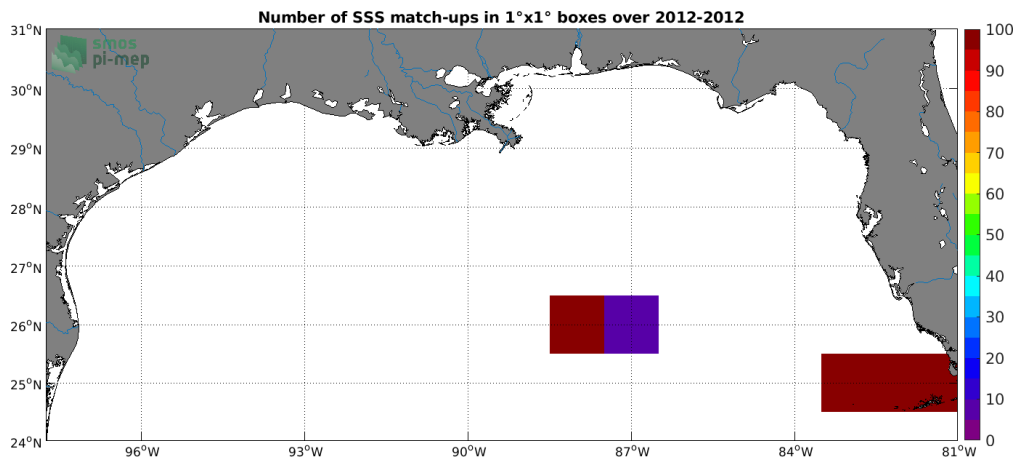
Figure 4: Number of SSS match-ups between TSG (GOSUD-Sailing-ship) SSS and the SMOS SSS L3 v2 - Daily - 0.5 Deg (CATDS-CECOS-IFREMER) SSS product for the Mississippi river plume Pi-MEP region over 1^\circ \times 1^\circ boxes and for the full satellite product period.
