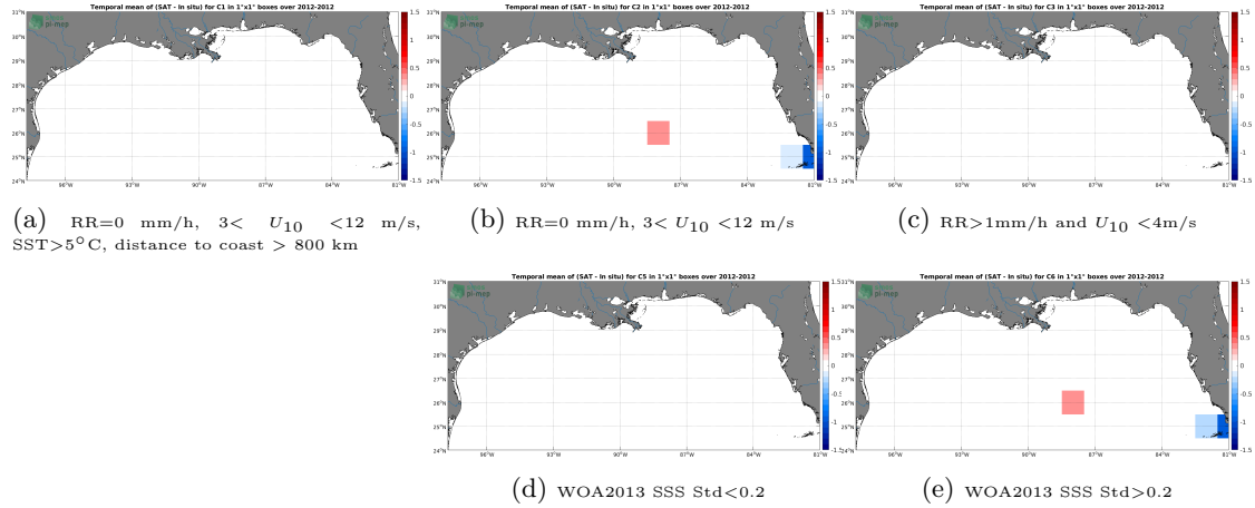
Figure 12: Temporal mean gridded over spatial boxes of size 1^{\circ}\times 1^{\circ} of \Delta SSS (SMOS SSS L3 v2 - Daily - 0.5 Deg (CATDS-CECOS-IFREMER) - TSG (GOSUD-Sailing-ship)) for 5 different subdatasets corresponding to:RR=0 mm/h, 3 < U_{10} < 12 m/s, SST >5^{\circ}\text{C} , distance to coast > 800 km (a), RR=0 mm/h, 3 < U_{10} < 12 m/s (b), RR >1 mm/h and U_{10} < 4 m/s (c), WOA2013 SSS Std <0.2 (d), WOA2013 SSS Std >0.2 (e).
