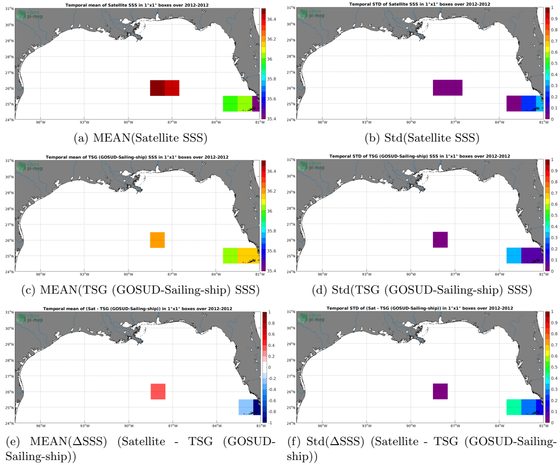
Figure 6: Temporal mean (left) and Std (right) of SSS from SMOS SSS L3 v2 - Daily - 0.5 Deg (CATDS-CECOS-IFREMER) (top), TSG (GOSUD-Sailing-ship) (middle), and of \Delta SSS (Satellite - TSG (GOSUD-Sailing-ship)). Only match-up pairs are used to generate these maps.
