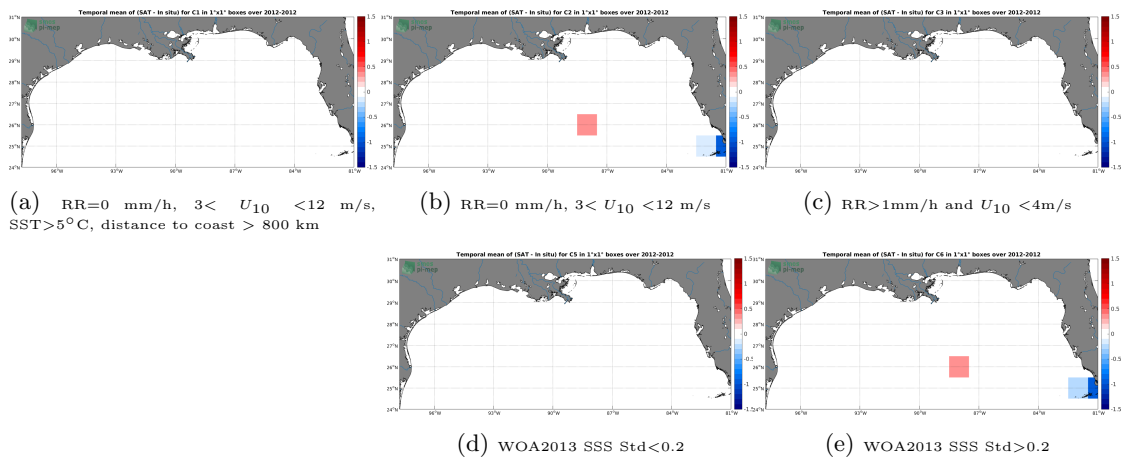
Figure 12: Temporal mean gridded over spatial boxes of size 1°x1° of \Delta SSS (SMOS-L3-CATDS-CECOS-IFREMER-V2-1DAY-0.5DEG - TSG-GOSUD-Sailing-ship) for 5 different subdatasets corresponding to:RR=0 mm/h, 3 < U_{10} < 12 m/s, SST>5°C, distance to coast > 800 km (a), RR=0 mm/h, 3 < U_{10} < 12 m/s (b), RR>1mm/h and U_{10} < 4 m/s (c), WOA2013 SSS Std<0.2 (d), WOA2013 SSS Std>0.2 (e).
