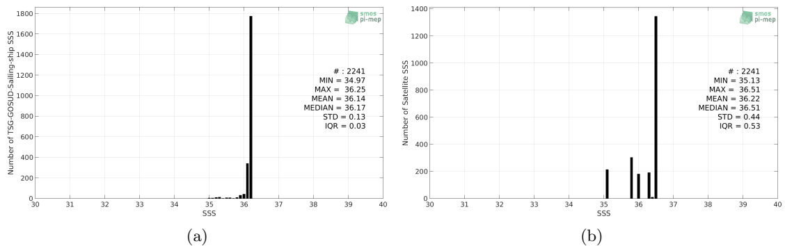
Figure 2: Histograms of SSS from TSG-GOSUD-Sailing-ship (a) and SMOS-L3-CATDS-CECOS-IFREMER-V2-1DAY-0.5DEG (b) considering all match-up pairs per bins of 0.1 over the Mississippi river plume Pi-MEP region and for the full satellite product period.
