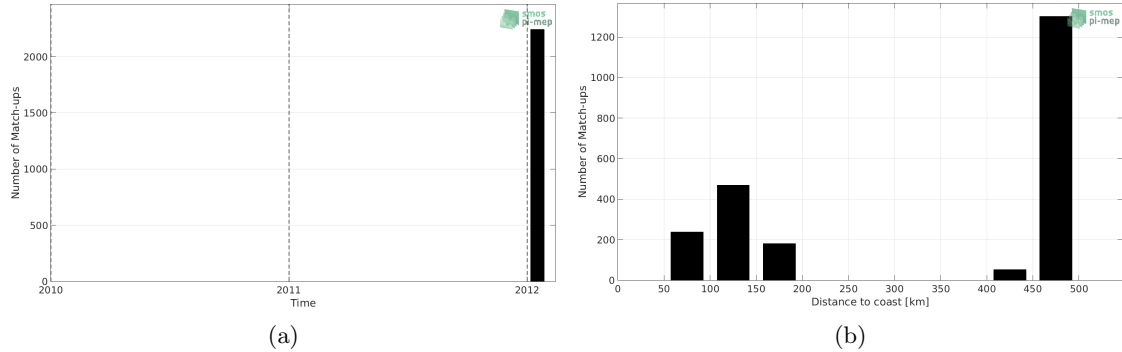
Figure 1: Number of match-ups between TSG-GOSUD-Sailing-ship and SMOS-L3-CATDS-CECOS-IFREMER-V2-1DAY-0.5DEG SSS as a function of time (a) and as function of the distance to coast (b) over the Mississippi river plume Pi-MEP region and for the full satellite product period.
