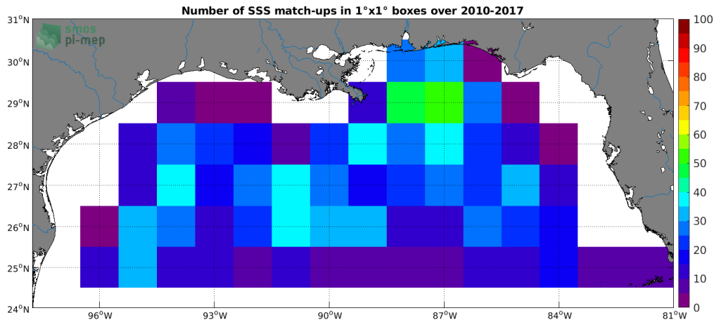
Figure 4: Number of SSS match-ups between Argo SSS and the SMOS SSS L3 v2 - Daily - 0.5 Deg (CATDS-CECOS-IFREMER) SSS product for the Mississippi river plume Pi-MEP region over 1^\circ \times 1^\circ boxes and for the full satellite product period.
