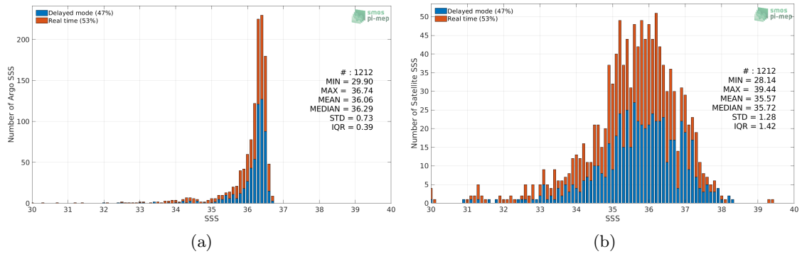
Figure 2: Histograms of SSS from Argo (a) and SMOS SSS L3 v2 - Daily - 0.5 Deg (CATDS-CECOS-IFREMER) (b) considering all match-up pairs per bins of 0.1 over the Mississippi river plume Pi-MEP region and for the full satellite product period.
