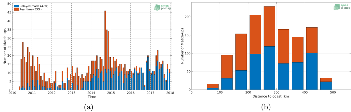
Figure 1: Number of match-ups between Argo and SMOS SSS L3 v2 - Daily - 0.5 Deg (CATDS-CECOS-IFREMER) SSS as a function of time (a) and as function of the distance to coast (b) over the Mississippi river plume Pi-MEP region and for the full satellite product period.
