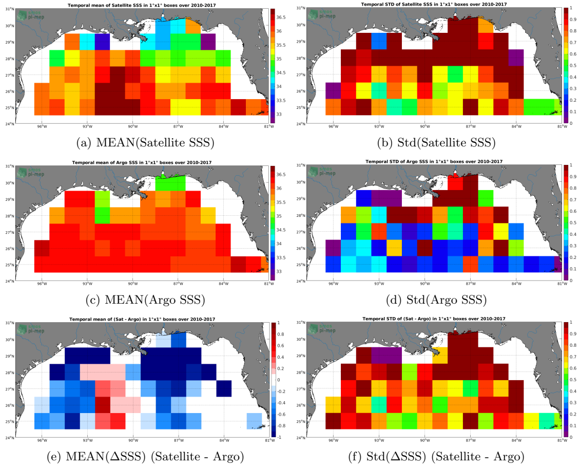
Figure 6: Temporal mean (left) and Std (right) of SSS from SMOS SSS L3 v2 - Daily - 0.5 Deg (CATDS-CECOS-IFREMER) (top), Argo (middle), and of \Delta SSS (Satellite - Argo). Only match-up pairs are used to generate these maps.
