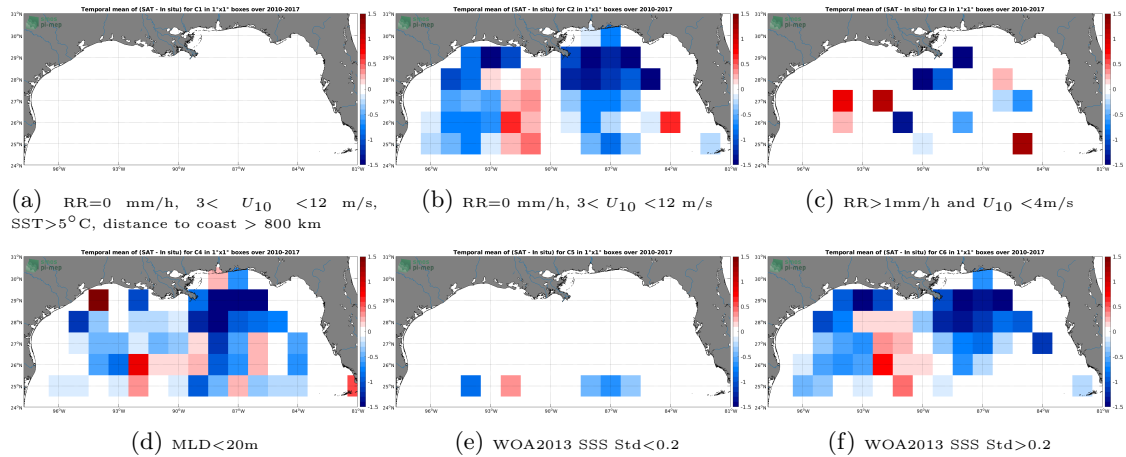
Figure 12: Temporal mean gridded over spatial boxes of size 1^{\circ}\times 1^{\circ} of \Delta\text{SSS} (SMOS SSS L3 v2 - Daily - 0.5 Deg (CATDS-CECOS-IFREMER) - Argo) for 6 different subdatasets corresponding to: RR=0 mm/h, 3 < U_{10} < 12 m/s, SST > 5^{\circ}\text{C} , distance to coast > 800 km (a), RR=0 mm/h, 3 < U_{10} < 12 m/s (b), RR > 1 mm/h and U_{10} < 4 m/s (c), MLD < 20 m (d), WOA2013 SSS Std < 0.2 (e), WOA2013 SSS Std > 0.2 (f).
