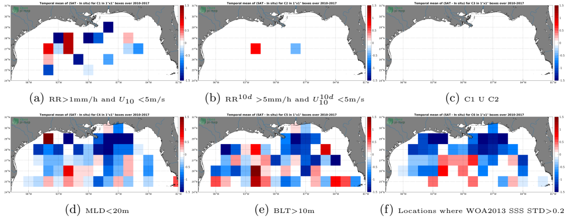
Figure 12: Temporal mean gridded over spatial boxes of size 1^\circ \times 1^\circ of \Delta\text{SSS} (SMOS-L3-CATDS-CECOS-IFREMER-V2-1DAY-0.5DEG - Argo) for 6 different subdatasets corresponding to: \text{RR} > 1\text{mm/h} and U_{10} < 5\text{m/s} (a), \text{RR}^{10d} > 5\text{mm/h} and U_{10}^{10d} < 5\text{m/s} (b), C1 U C2 (c), \text{MLD} < 20\text{m} (d), \text{BLT} > 10\text{m} (e), Locations where WOA2013 SSS \text{STD} > 0.2 (f).
