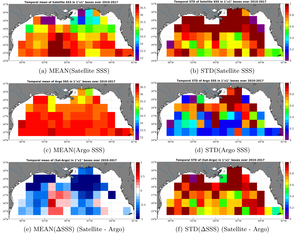
Figure 6: Temporal mean (left) and STD (right) of SSS from SMOS-L3-CATDS-CECOS-IFREMER-V2-1DAY-0.5DEG (top), Argo (middle), and of \Delta\text{SSS}(\text{Satellite} - \text{Argo}) . Only match-up pairs are used to generate these maps.
