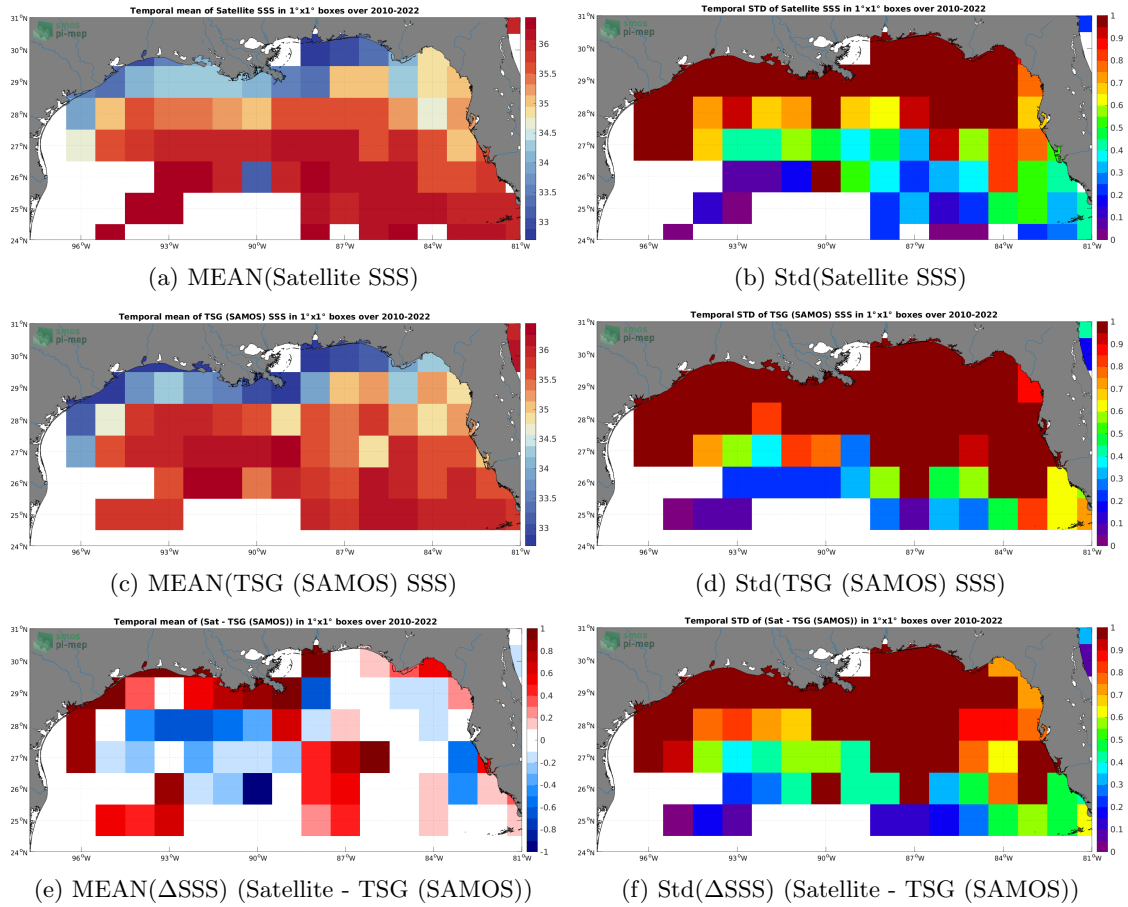
Figure 6: Temporal mean (left) and Std (right) of SSS from SMOS SSS L3 v335 - Monthly - 25 km (CATDS-CPDC) (top), TSG (SAMOS) (middle), and of \Delta SSS (Satellite - TSG (SAMOS)). Only match-up pairs are used to generate these maps.
