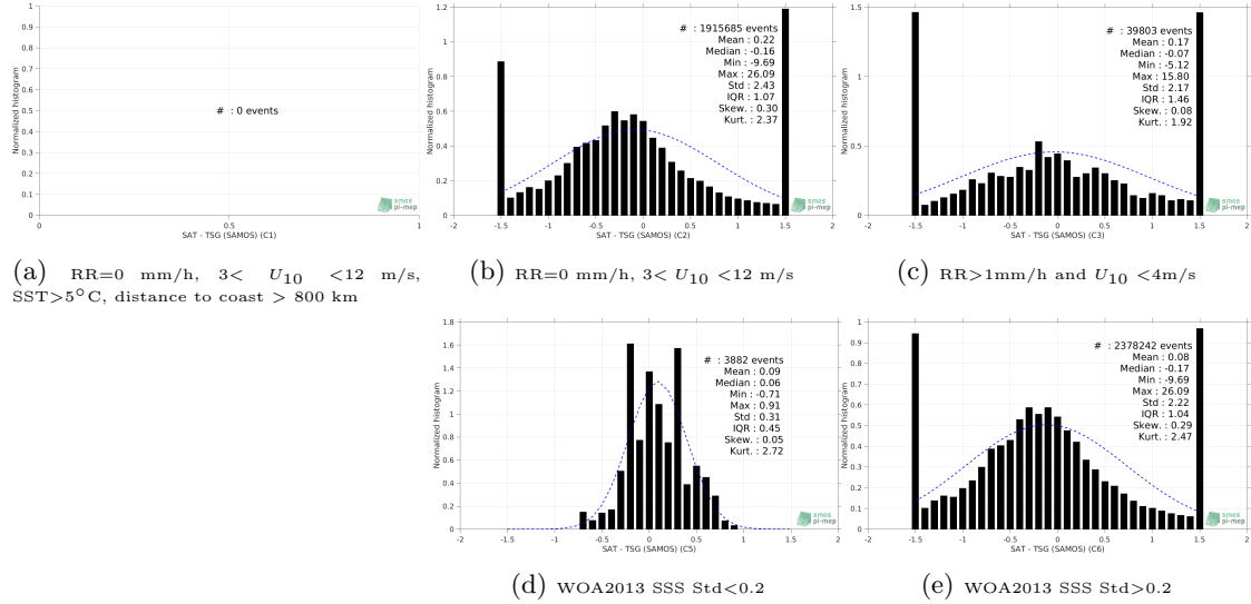
Figure 13: Normalized histogram of \Delta\text{SSS} (SMOS SSS L3 v335 - Monthly - 25 km (CATDS-CPDC) - TSG (SAMOS)) for 5 different subdatasets corresponding to: RR=0 mm/h, 3 < U_{10} < 12 m/s, SST > 5^\circ\text{C} , distance to coast > 800 km (a), RR=0 mm/h, 3 < U_{10} < 12 m/s (b), RR > 1 mm/h and U_{10} < 4 m/s (c), WOA2013 SSS Std < 0.2 (d), WOA2013 SSS Std > 0.2 (e).
