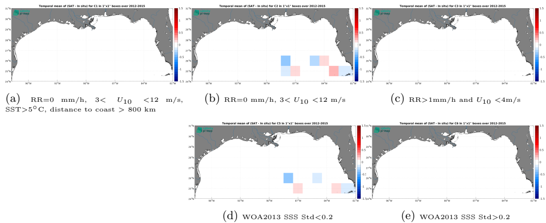
Figure 14: Temporal mean gridded over spatial boxes of size 1^\circ \times 1^\circ of \Delta SSS (SMOS SSS L3 v335 - Monthly - 25 km (CATDS-CPDC) - TSG (GOSUD-Sailing-ship)) for 5 different subdatasets corresponding to: RR=0 mm/h, 3 < U_{10} < 12 m/s, SST > 5^\circ\text{C} , distance to coast > 800 km (a), RR=0 mm/h, 3 < U_{10} < 12 m/s (b), RR > 1 mm/h and U_{10} < 4 m/s (c), WOA2013 SSS Std < 0.2 (d), WOA2013 SSS Std > 0.2 (e).
