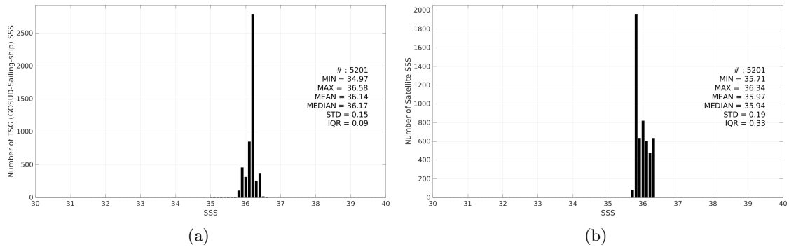
Figure 3: Histograms of SSS from TSG (GOSUD-Sailing-ship) (a) and SMOS SSS L3 v335 - Monthly - 25 km (CATDS-CPDC) (b) considering all match-up pairs per bins of 0.1 over the Mississippi river plume Pi-MEP region and for the full satellite product period.
