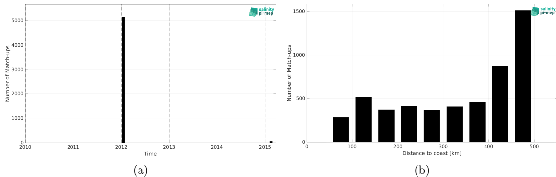
Figure 2: Number of match-ups between TSG (GOSUD-Sailing-ship) and SMOS SSS L3 v335 - Monthly - 25 km (CATDS-CPDC) SSS as a function of time (a) and as function of the distance to coast (b) over the Mississippi river plume Pi-MEP region and for the full satellite product period.
