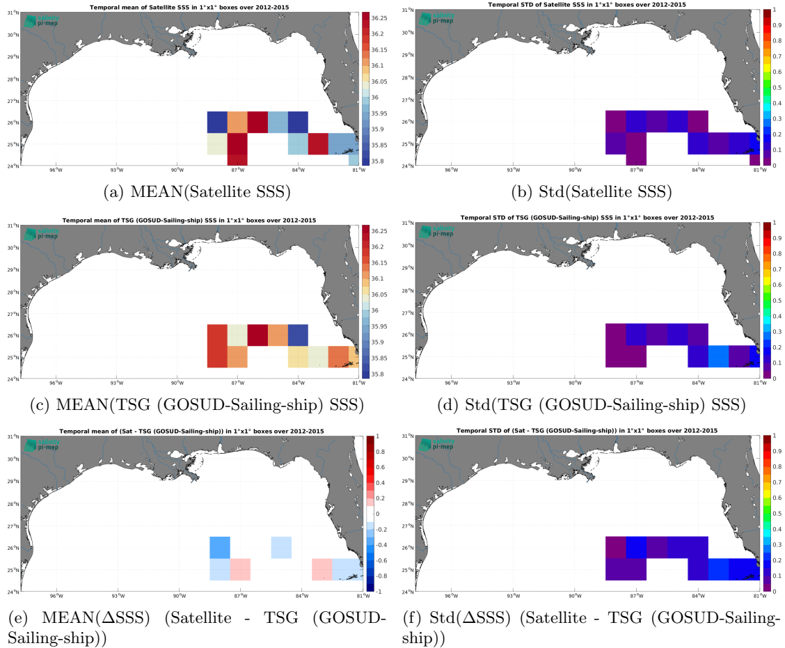
Figure 7: Temporal mean (left) and Std (right) of SSS from SMOS SSS L3 v335 - Monthly - 25 km (CATDS-CPDC) (top), TSG (GOSUD-Sailing-ship) (middle), and of \Delta\text{SSS} (Satellite - TSG (GOSUD-Sailing-ship)). Only match-up pairs are used to generate these maps.
