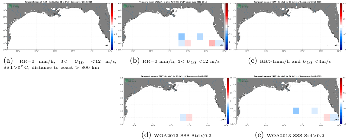
Figure 12: Temporal mean gridded over spatial boxes of size 1^{\circ}\times 1^{\circ} of \Delta SSS (SMOS SSS L3 v335 - Monthly - 25 km (CATDS-CPDC) - TSG (GOSUD-Sailing-ship)) for 5 different subdatasets corresponding to:RR=0 mm/h, 3 < U_{10} < 12 m/s, SST >5^{\circ}\text{C} , distance to coast > 800 km (a), RR=0 mm/h, 3 < U_{10} < 12 m/s (b), RR >1 mm/h and U_{10} < 4 m/s (c), WOA2013 SSS Std <0.2 (d), WOA2013 SSS Std >0.2 (e).
