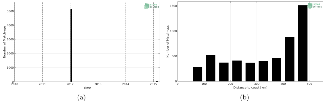
Figure 1: Number of match-ups between TSG (GOSUD-Sailing-ship) and SMOS SSS L3 v335 - Monthly - 25 km (CATDS-CPDC) SSS as a function of time (a) and as function of the distance to coast (b) over the Mississippi river plume Pi-MEP region and for the full satellite product period.
