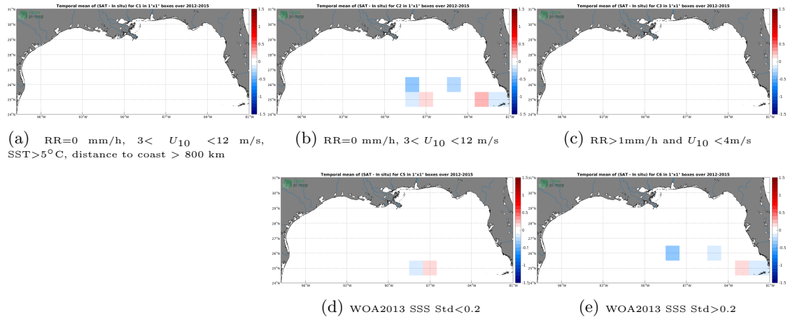
Figure 12: Temporal mean gridded over spatial boxes of size 1^\circ \times 1^\circ of \Delta SSS (SMOS SSS L3 v335 - Monthly - 25 km (CATDS-CPDC) - TSG (GOSUD-Sailing-ship)) for 5 different subdatasets corresponding to: RR=0 mm/h, 3 < U_{10} < 12 m/s, SST > 5^\circ\text{C} , distance to coast > 800 km (a), RR=0 mm/h, 3 < U_{10} < 12 m/s (b), RR > 1 mm/h and U_{10} < 4 m/s (c), WOA2013 SSS Std < 0.2 (d), WOA2013 SSS Std > 0.2 (e).
