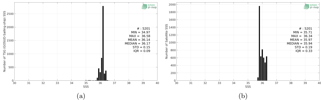
Figure 2: Histograms of SSS from TSG (GOSUD-Sailing-ship) (a) and SMOS SSS L3 v335 - Monthly - 25 km (CATDS-CPDC) (b) considering all match-up pairs per bins of 0.1 over the Mississippi river plume Pi-MEP region and for the full satellite product period.
