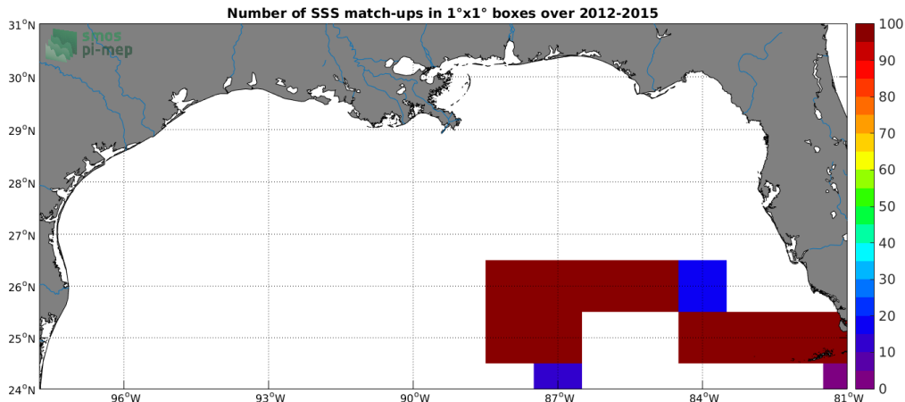
Figure 4: Number of SSS match-ups between TSG (GOSUD-Sailing-ship) SSS and the SMOS SSS L3 v335 - Monthly - 25 km (CATDS-CPDC) SSS product for the Mississippi river plume Pi-MEP region over 1^\circ \times 1^\circ boxes and for the full satellite product period.
