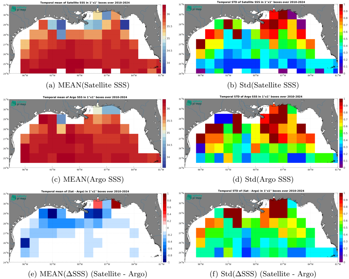
Figure 7: Temporal mean (left) and Std (right) of SSS from SMOS SSS L3 v335 - Monthly - 25 km (CATDS-CPDC) (top), Argo (middle), and of \Delta\text{SSS} (Satellite - Argo). Only match-up pairs are used to generate these maps.
