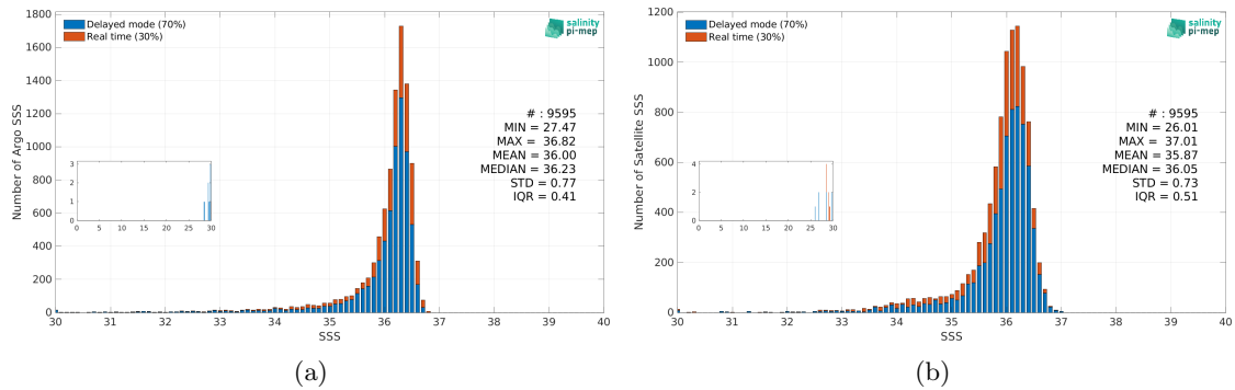
Figure 3: Histograms of SSS from Argo (a) and SMOS SSS L3 v335 - Monthly - 25 km (CATDS-CPDC) (b) considering all match-up pairs per bins of 0.1 over the Mississippi river plume Pi-MEP region and for the full satellite product period.
