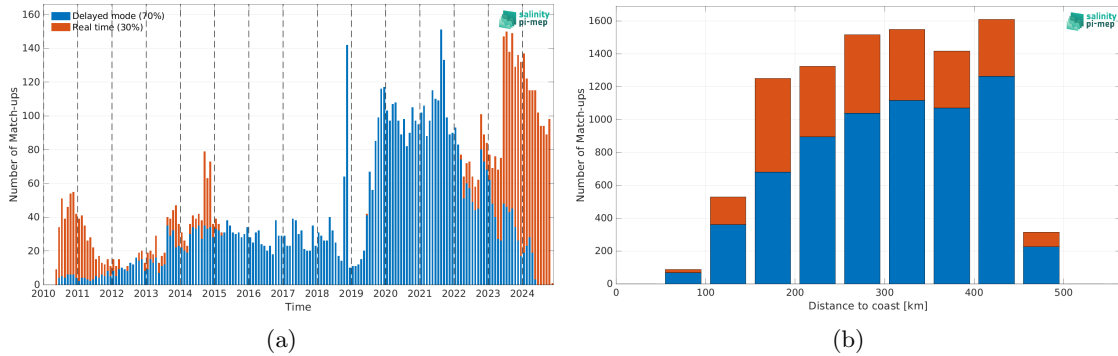
Figure 2: Number of match-ups between Argo and SMOS SSS L3 v335 - Monthly - 25 km (CATDS-CPDC) SSS as a function of time (a) and as function of the distance to coast (b) over the Mississippi river plume Pi-MEP region and for the full satellite product period.
