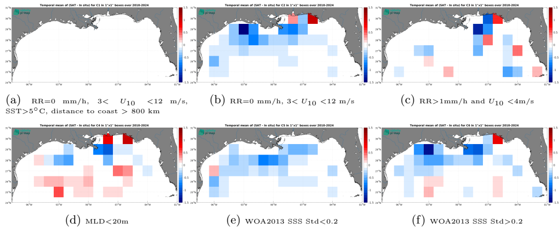
Figure 14: Temporal mean gridded over spatial boxes of size 1^\circ \times 1^\circ of \Delta SSS (SMOS SSS L3 v335 - Monthly - 25 km (CATDS-CPDC) - Argo) for 6 different subdatasets corresponding to: RR=0 mm/h, 3 < U_{10} < 12 m/s, SST > 5^\circ\text{C} , distance to coast > 800 km (a), RR=0 mm/h, 3 < U_{10} < 12 m/s (b), RR > 1 mm/h and U_{10} < 4 m/s (c), MLD < 20 m (d), WOA2013 SSS Std < 0.2 (e), WOA2013 SSS Std > 0.2 (f).
