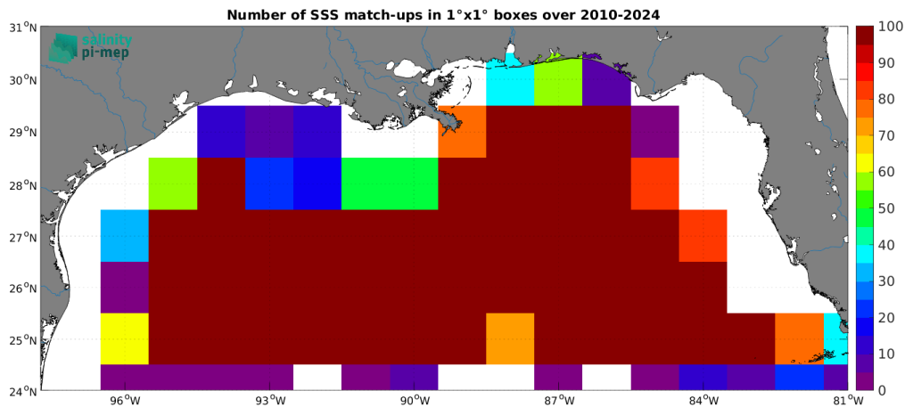
Figure 5: Number of SSS match-ups between Argo SSS and the SMOS SSS L3 v335 - Monthly - 25 km (CATDS-CPDC) SSS product for the Mississippi river plume Pi-MEP region over 1^\circ \times 1^\circ boxes and for the full satellite product period.
