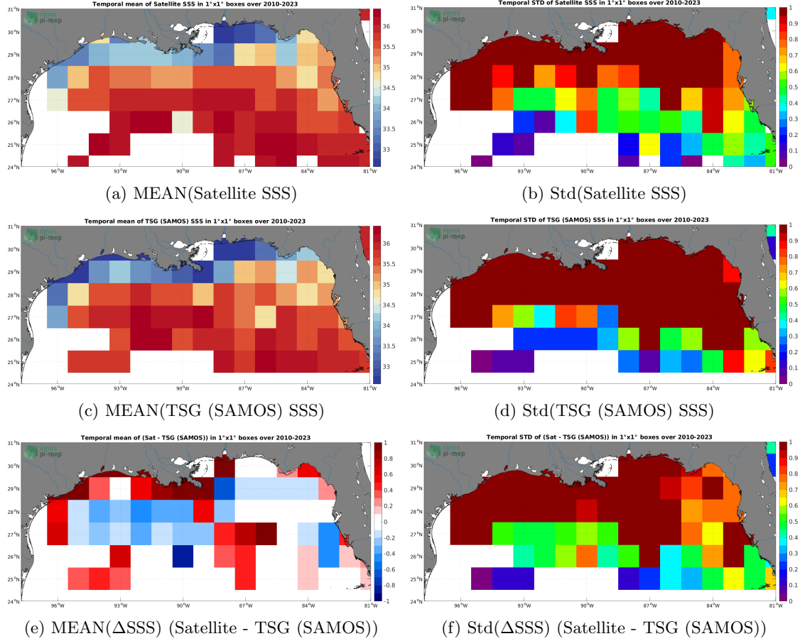
Figure 6: Temporal mean (left) and Std (right) of SSS from SMOS SSS L3 v335 - 10 Days - 25 km (CATDS-CPDC) (top), TSG (SAMOS) (middle), and of \Delta\text{SSS} (Satellite - TSG (SAMOS)). Only match-up pairs are used to generate these maps.
