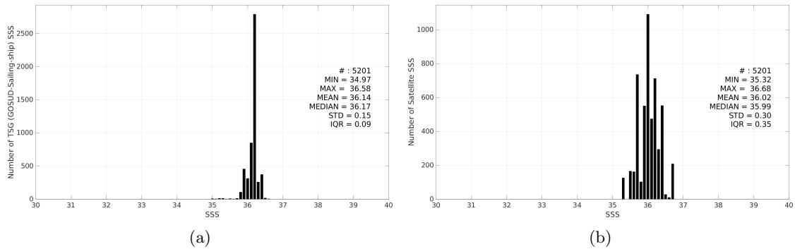
Figure 3: Histograms of SSS from TSG (GOSUD-Sailing-ship) (a) and SMOS SSS L3 v335 - 10 Days - 25 km (CATDS-CPDC) (b) considering all match-up pairs per bins of 0.1 over the Mississippi river plume Pi-MEP region and for the full satellite product period.
