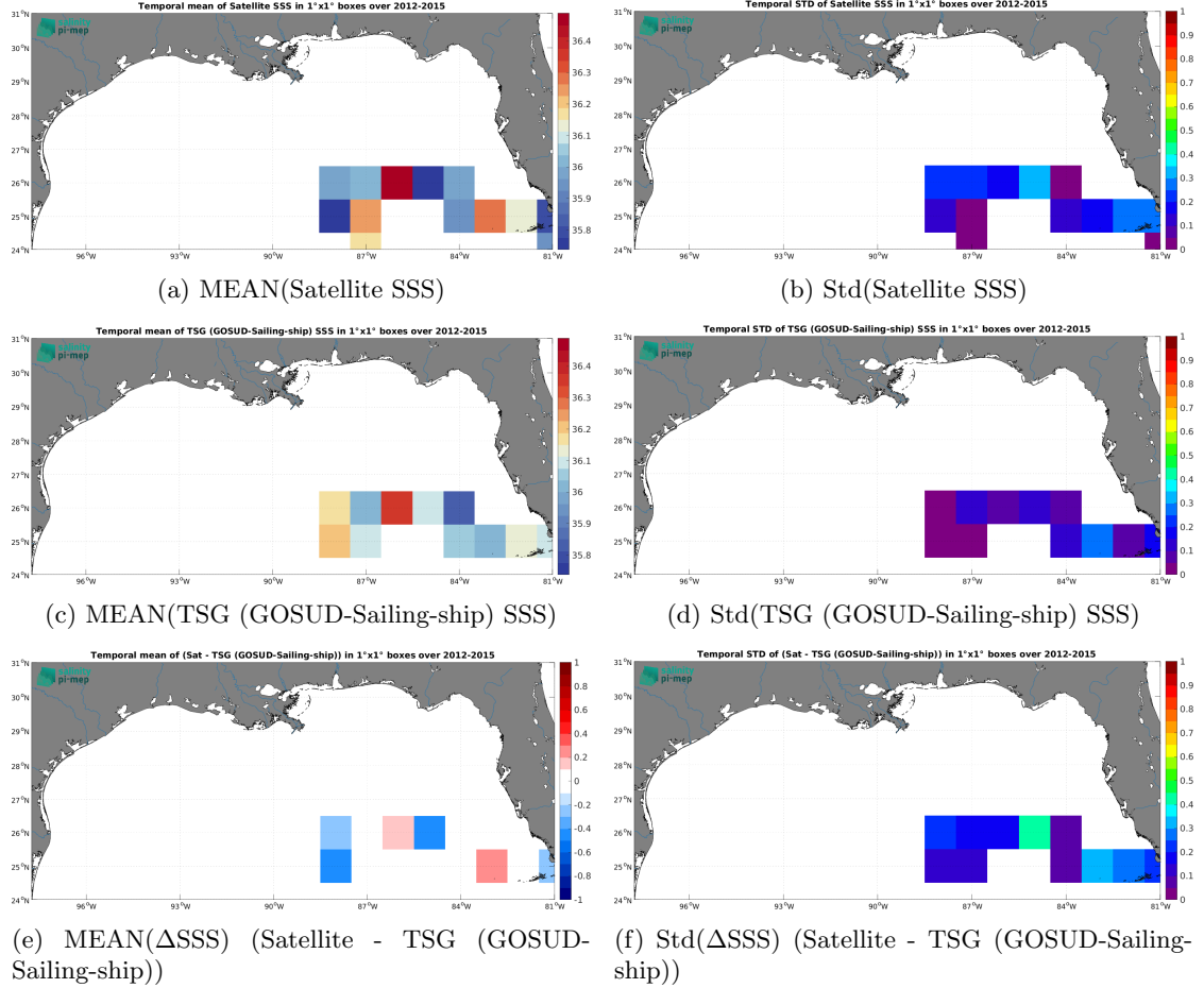
Figure 7: Temporal mean (left) and Std (right) of SSS from SMOS SSS L3 v335 - 10 Days - 25 km (CATDS-CPDC) (top), TSG (GOSUD-Sailing-ship) (middle), and of \Delta\text{SSS} (Satellite - TSG (GOSUD-Sailing-ship)). Only match-up pairs are used to generate these maps.
