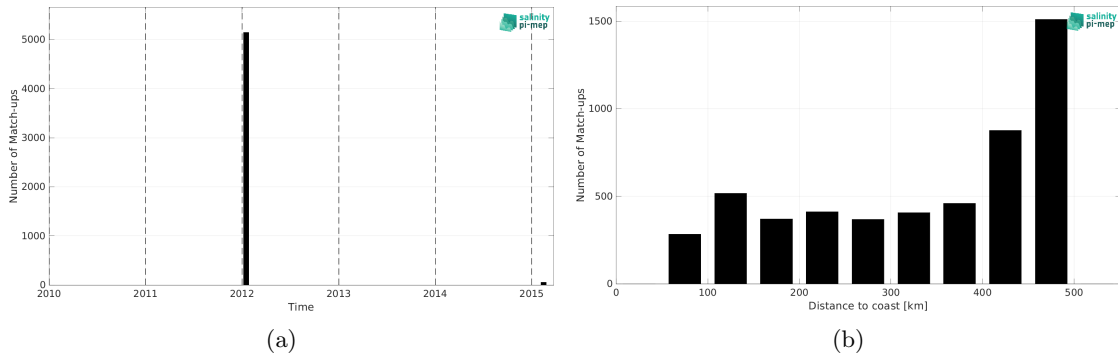
Figure 2: Number of match-ups between TSG (GOSUD-Sailing-ship) and SMOS SSS L3 v335 - 10 Days - 25 km (CATDS-CPDC) SSS as a function of time (a) and as function of the distance to coast (b) over the Mississippi river plume Pi-MEP region and for the full satellite product period.
