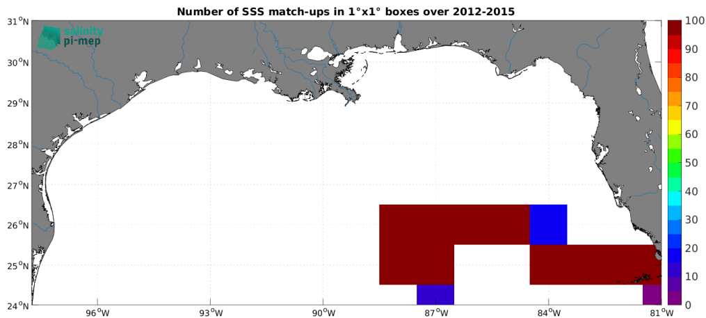
Figure 5: Number of SSS match-ups between TSG (GOSUD-Sailing-ship) SSS and the SMOS SSS L3 v335 - 10 Days - 25 km (CATDS-CPDC) SSS product for the Mississippi river plume Pi-MEP region over 1^\circ \times 1^\circ boxes and for the full satellite product period.
