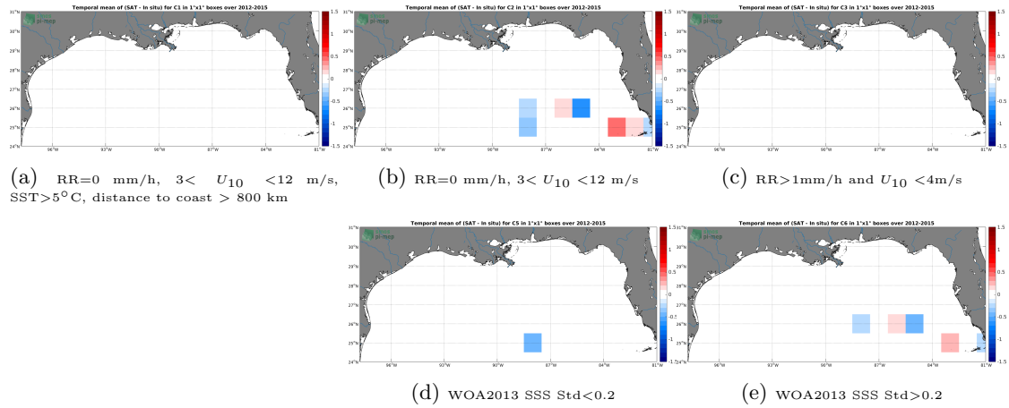
Figure 12: Temporal mean gridded over spatial boxes of size 1^\circ \times 1^\circ of \Delta SSS (SMOS SSS L3 v335 - 10 Days - 25 km (CATDS-CPDC) - TSG (GOSUD-Sailing-ship)) for 5 different subdatasets corresponding to: RR=0 mm/h, 3 < U_{10} < 12 m/s, SST > 5^\circ\text{C} , distance to coast > 800 km (a), RR=0 mm/h, 3 < U_{10} < 12 m/s (b), RR > 1 mm/h and U_{10} < 4 m/s (c), WOA2013 SSS Std < 0.2 (d), WOA2013 SSS Std > 0.2 (e).
