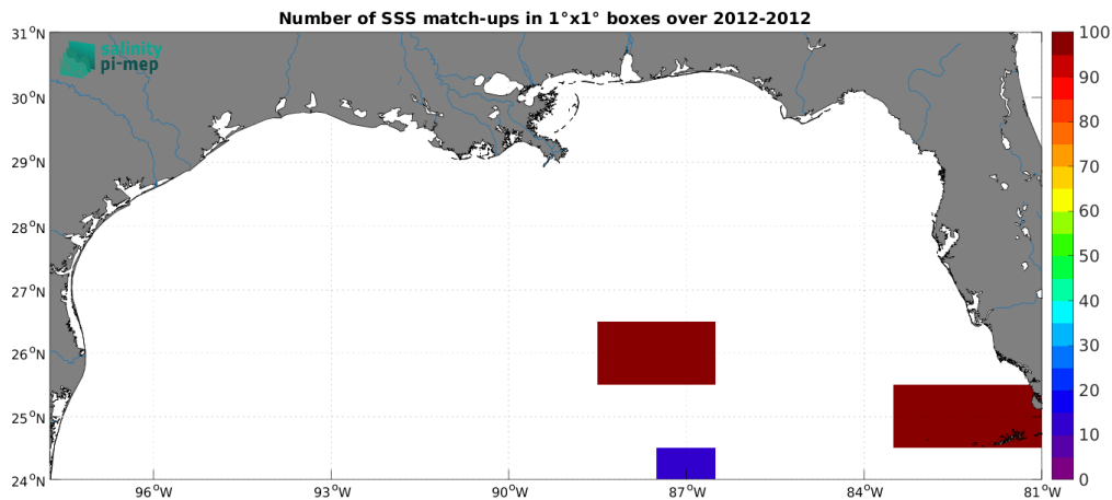
Figure 5: Number of SSS match-ups between TSG (GOSUD-Sailing-ship) SSS and the SMOS SSS L2Q v333 - 0.25 Deg (CATDS-CPDC) SSS product for the Mississippi river plume Pi-MEP region over 1^\circ \times 1^\circ boxes and for the full satellite product period.
