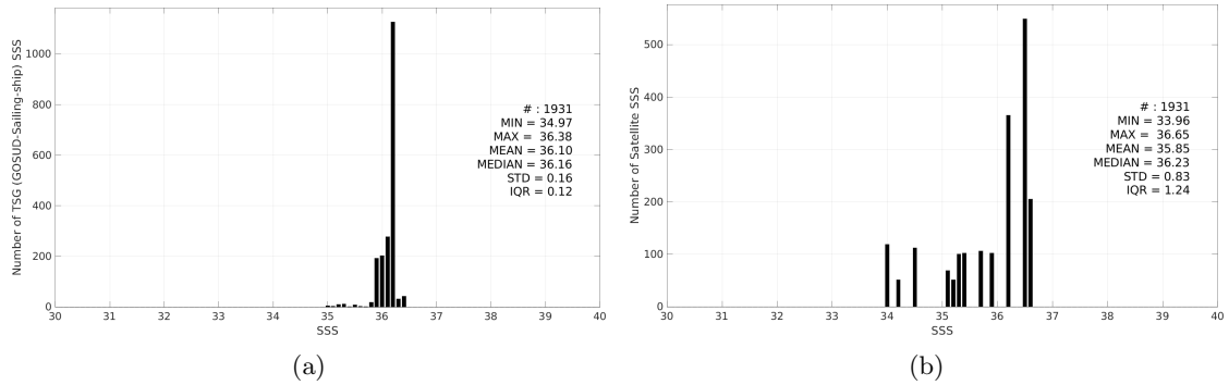
Figure 3: Histograms of SSS from TSG (GOSUD-Sailing-ship) (a) and SMOS SSS L2Q v333 - 0.25 Deg (CATDS-CPDC) (b) considering all match-up pairs per bins of 0.1 over the Mississippi river plume Pi-MEP region and for the full satellite product period.
