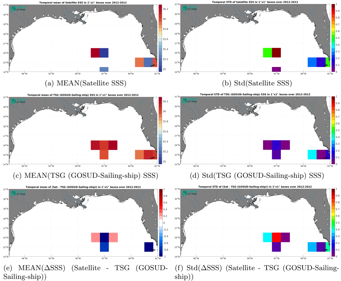
Figure 7: Temporal mean (left) and Std (right) of SSS from SMOS SSS L2Q v333 - 0.25 Deg (CATDS-CPDC) (top), TSG (GOSUD-Sailing-ship) (middle), and of \Delta\text{SSS} (Satellite - TSG (GOSUD-Sailing-ship)). Only match-up pairs are used to generate these maps.
