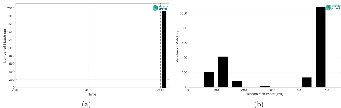
Figure 2: Number of match-ups between TSG (GOSUD-Sailing-ship) and SMOS SSS L2Q v333 - 0.25 Deg (CATDS-CPDC) SSS as a function of time (a) and as function of the distance to coast (b) over the Mississippi river plume Pi-MEP region and for the full satellite product period.
