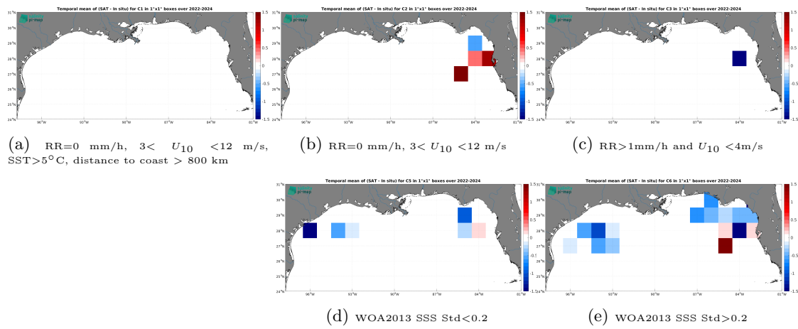
Figure 14: Temporal mean gridded over spatial boxes of size 1^\circ \times 1^\circ of \Delta SSS (SMOS SSS L2Q v333 - 0.25 Deg (CATDS-CPDC) - Sailability) for 5 different subdatasets corresponding to: RR=0 mm/h, 3 < U_{10} < 12 m/s, SST > 5°C, distance to coast > 800 km (a), RR=0 mm/h, 3 < U_{10} < 12 m/s (b), RR > 1mm/h and U_{10} < 4 m/s (c), WOA2013 SSS Std < 0.2 (d), WOA2013 SSS Std > 0.2 (e).
