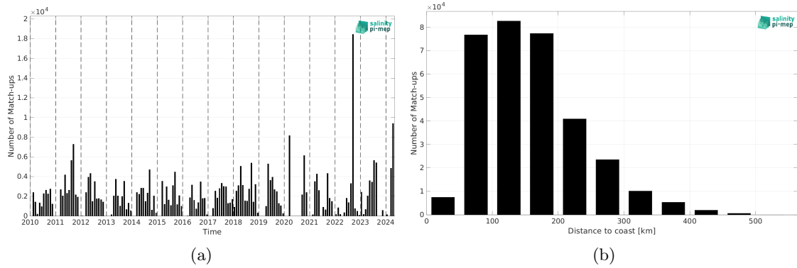
Figure 2: Number of match-ups between TSG (SAMOS) and SMOS SSS L3 v332 - 9 Days (CATDS-CPDC) SSS as a function of time (a) and as function of the distance to coast (b) over the Mississippi river plume Pi-MEP region and for the full satellite product period.
