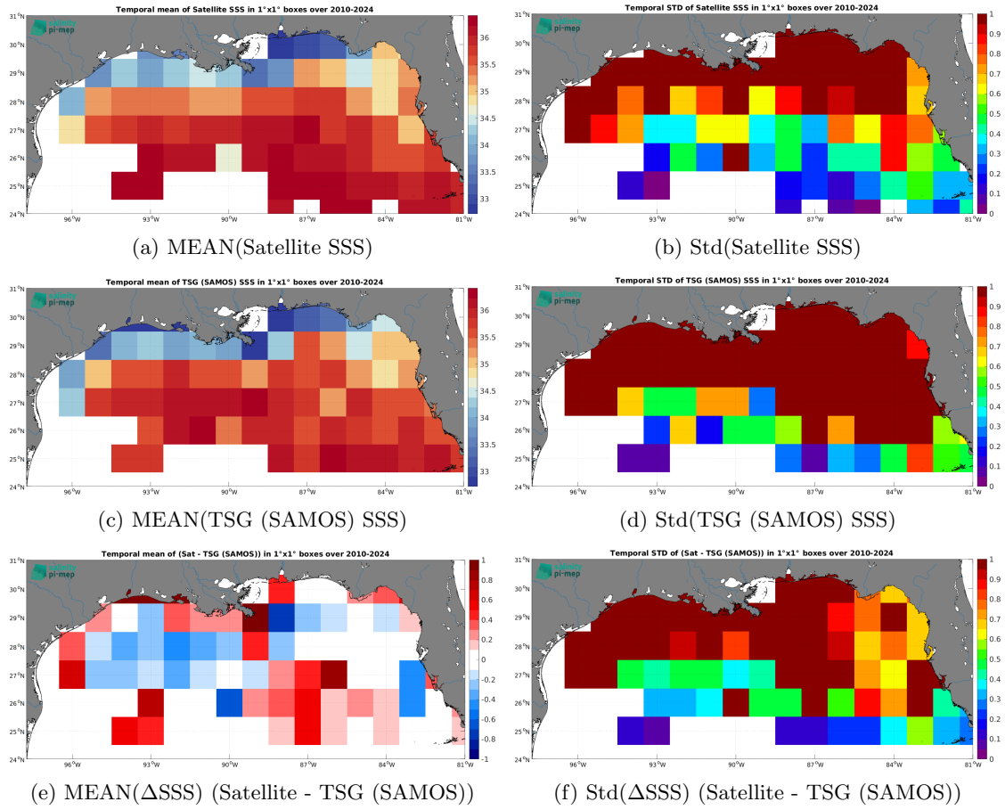
Figure 7: Temporal mean (left) and Std (right) of SSS from SMOS SSS L3 v332 - 9 Days (CATDS-CPDC) (top), TSG (SAMOS) (middle), and of \Delta SSS (Satellite - TSG (SAMOS)). Only match-up pairs are used to generate these maps.
