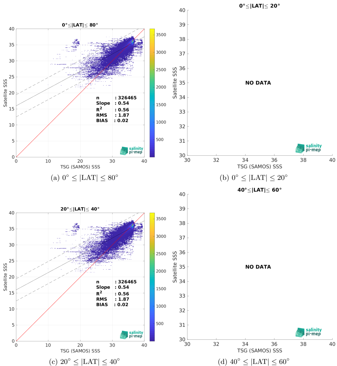
Figure 10: Contour maps of the concentration of SMOS SSS L3 v332 - 9 Days (CATDS-CPDC) SSS (y-axis) versus TSG (SAMOS) SSS (x-axis) at match-up pairs for different latitude bands. For each plot, the red line shows x=y . The black thin and dashed lines indicate a linear fit through the data cloud and the \pm 95\% confidence levels, respectively. The number match-up pairs n , the slope and R^2 coefficient of the linear fit, the root mean square (RMS) and the mean bias between satellite and in situ data are indicated for each latitude band in each plot.
