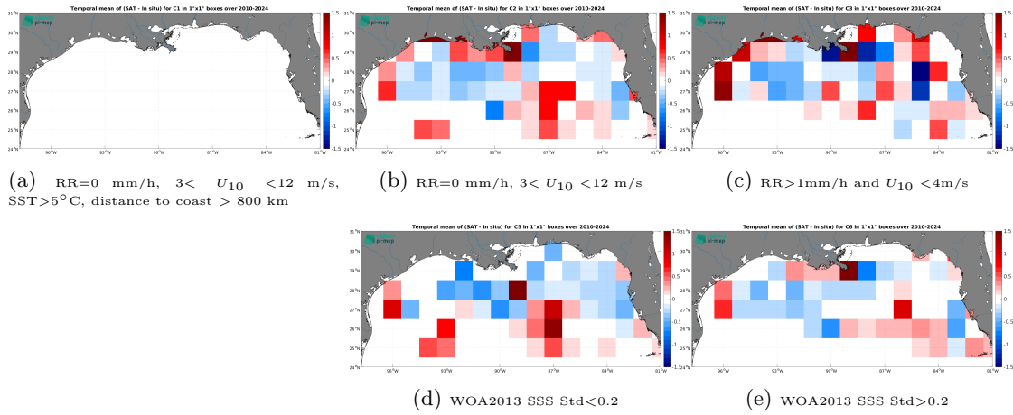
Figure 14: Temporal mean gridded over spatial boxes of size 1^\circ \times 1^\circ of \Delta SSS (SMOS SSS L3 v332 - 9 Days (CATDS-CPDC) - TSG (SAMOS)) for 5 different subdatasets corresponding to:RR=0 mm/h, 3 < U_{10} < 12 m/s, SST > 5°C, distance to coast > 800 km (a), RR=0 mm/h, 3 < U_{10} < 12 m/s (b), RR > 1mm/h and U_{10} < 4 m/s (c), WOA2013 SSS Std < 0.2 (d), WOA2013 SSS Std > 0.2 (e).
