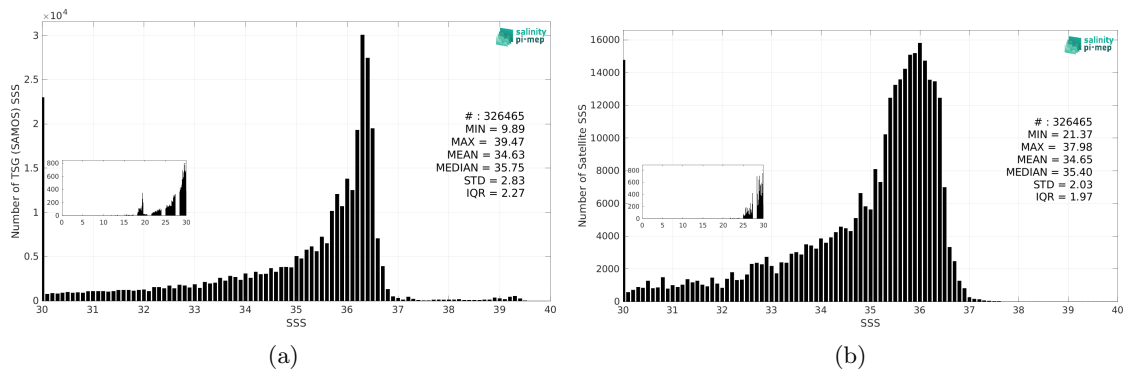
Figure 3: Histograms of SSS from TSG (SAMOS) (a) and SMOS SSS L3 v332 - 9 Days (CATDS-CPDC) (b) considering all match-up pairs per bins of 0.1 over the Mississippi river plume Pi-MEP region and for the full satellite product period.
