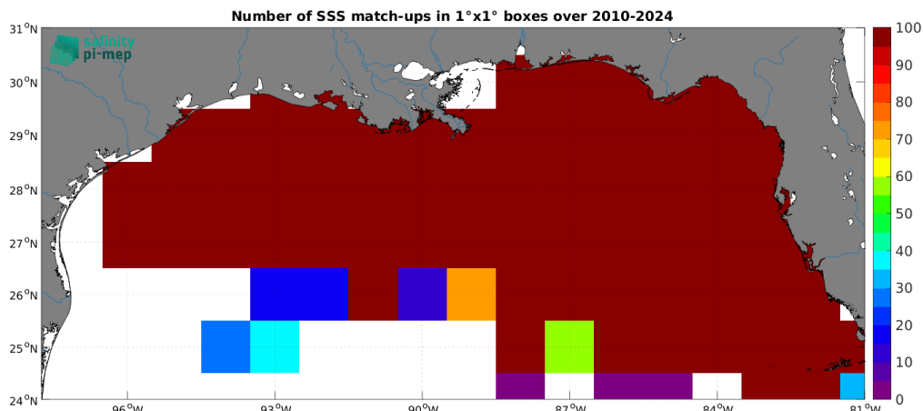
Figure 5: Number of SSS match-ups between TSG (SAMOS) SSS and the SMOS SSS L3 v332 - 9 Days (CATDS-CPDC) SSS product for the Mississippi river plume Pi-MEP region over 1^\circ \times 1^\circ boxes and for the full satellite product period.
