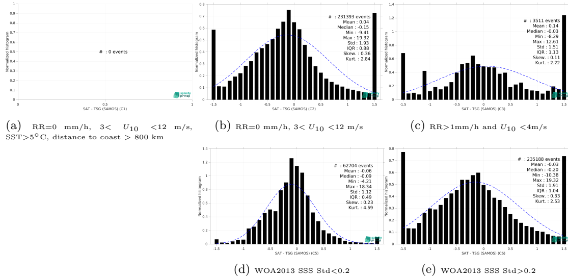
Figure 15: Normalized histogram of \Delta SSS (SMOS SSS L3 v332 - 9 Days (CATDS-CPDC) - TSG (SAMOS)) for 5 different subdatasets corresponding to: RR=0 mm/h, 3 < U_{10} < 12 m/s, SST>5°C, distance to coast > 800 km (a), RR=0 mm/h, 3 < U_{10} < 12 m/s (b), RR>1mm/h and U_{10} < 4 m/s (c), WOA2013 SSS Std<0.2 (d), WOA2013 SSS Std>0.2 (e).
