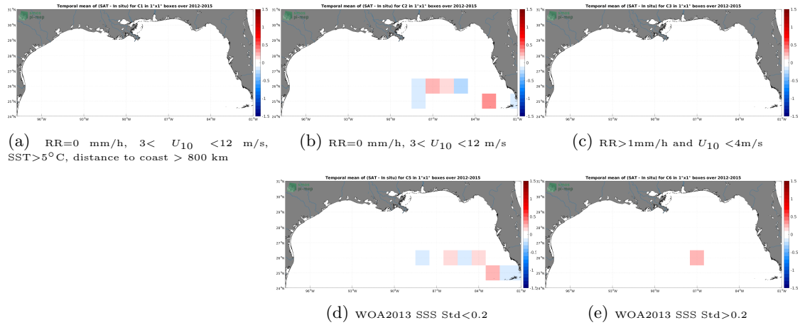
Figure 12: Temporal mean gridded over spatial boxes of size 1^{\circ}\times 1^{\circ} of \Delta SSS (SMOS SSS L3 v332 - 9 Days (CATDS-CPDC) - TSG (GOSUD-Sailing-ship)) for 5 different subdatasets corresponding to:RR=0 mm/h, 3 < U_{10} < 12 m/s, SST >5^{\circ}\text{C} , distance to coast > 800 km (a), RR=0 mm/h, 3 < U_{10} < 12 m/s (b), RR >1 mm/h and U_{10} < 4 m/s (c), WOA2013 SSS Std <0.2 (d), WOA2013 SSS Std >0.2 (e).
