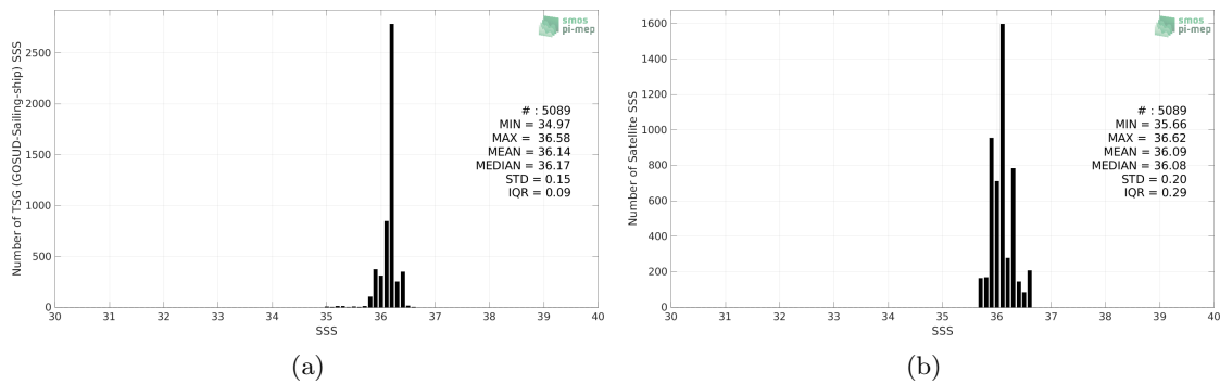
Figure 2: Histograms of SSS from TSG (GOSUD-Sailing-ship) (a) and SMOS SSS L3 v332 - 9 Days (CATDS-CPDC) (b) considering all match-up pairs per bins of 0.1 over the Mississippi river plume Pi-MEP region and for the full satellite product period.
