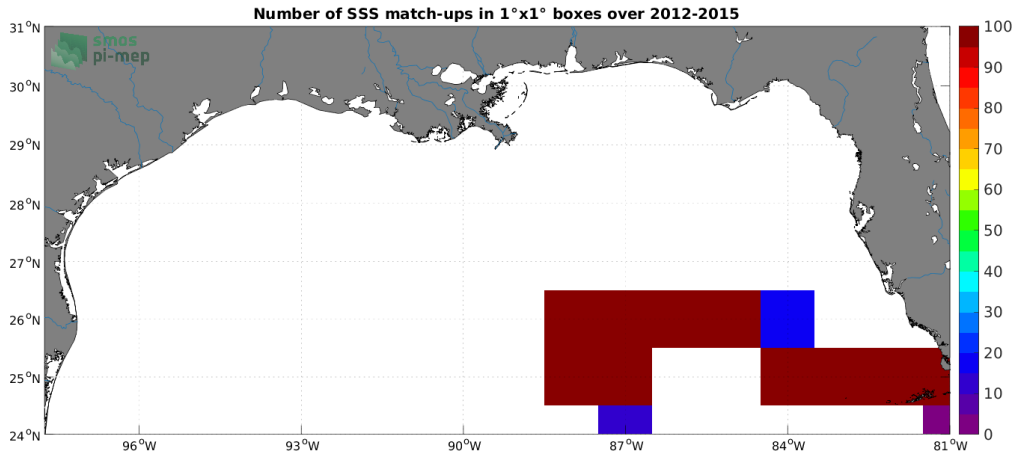
Figure 4: Number of SSS match-ups between TSG (GOSUD-Sailing-ship) SSS and the SMOS SSS L3 v332 - 9 Days (CATDS-CPDC) SSS product for the Mississippi river plume Pi-MEP region over 1^\circ \times 1^\circ boxes and for the full satellite product period.
