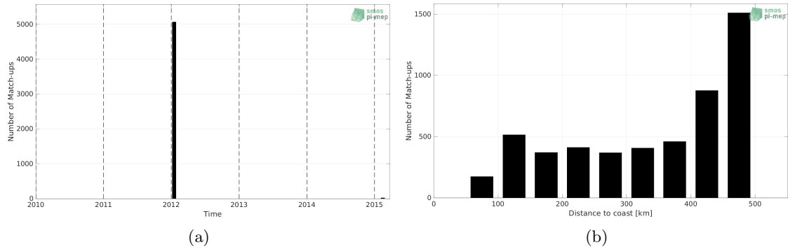
Figure 1: Number of match-ups between TSG (GOSUD-Sailing-ship) and SMOS SSS L3 v332 - 9 Days (CATDS-CPDC) SSS as a function of time (a) and as function of the distance to coast (b) over the Mississippi river plume Pi-MEP region and for the full satellite product period.
