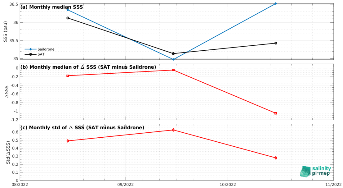
Figure 7: Time series of the monthly median SSS (top), median of \Delta SSS (Satellite - Sairdron) and Std of \Delta SSS (Satellite - Sairdron) over the Mississippi river plume Pi-MEP region considering all match-ups collected by the Pi-MEP.
