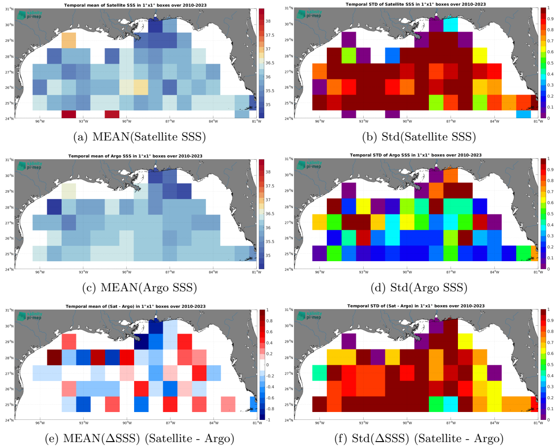
Figure 6: Temporal mean (left) and Std (right) of SSS from SMOS SSS L2Q v331 - 0.25 Deg (CATDS-CPDC) (top), Argo (middle), and of \Delta SSS (Satellite - Argo). Only match-up pairs are used to generate these maps.
