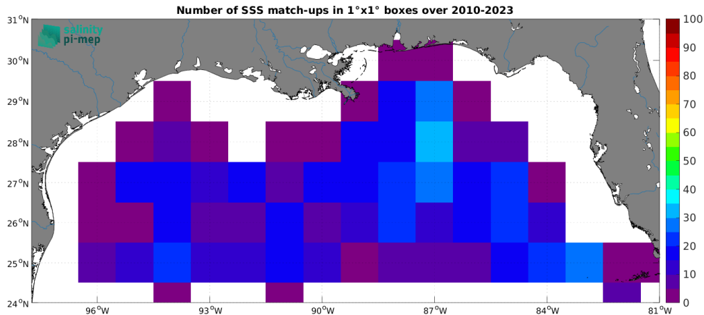
Figure 4: Number of SSS match-ups between Argo SSS and the SMOS SSS L2Q v331 - 0.25 Deg (CATDS-CPDC) SSS product for the Mississippi river plume Pi-MEP region over 1^\circ \times 1^\circ boxes and for the full satellite product period.
