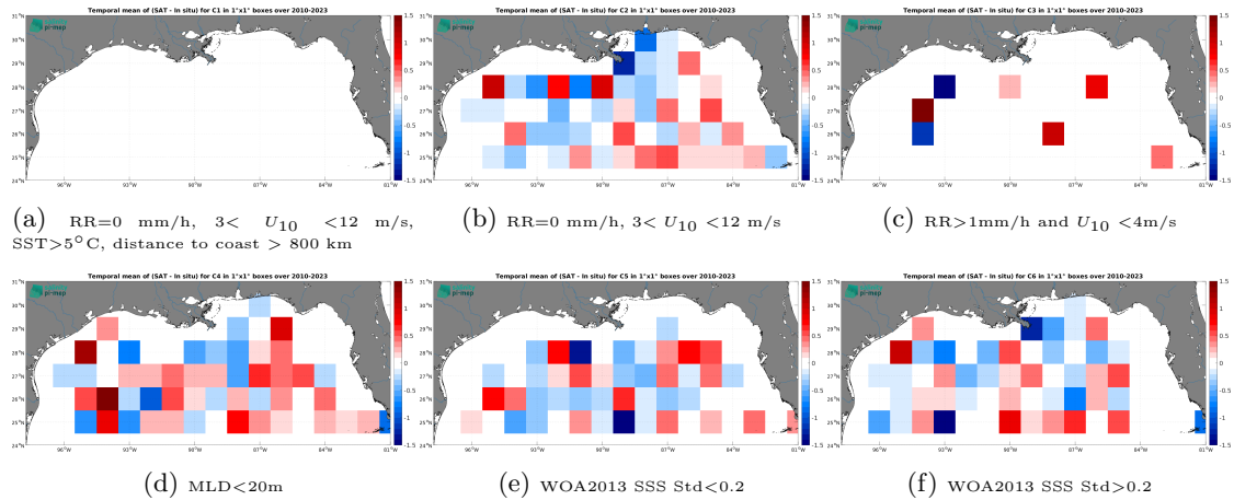
Figure 12: Temporal mean gridded over spatial boxes of size 1^{\circ}\times 1^{\circ} of \Delta\text{SSS} (SMOS SSS L2Q v331 - 0.25 Deg (CATDS-CPDC) - Argo) for 6 different subdatasets corresponding to:RR=0 mm/h, 3 < U_{10} < 12 m/s, SST > 5^{\circ}\text{C} , distance to coast > 800 km (a), RR=0 mm/h, 3 < U_{10} < 12 m/s (b), RR > 1\text{mm/h} and U_{10} < 4\text{m/s} (c),MLD < 20\text{m} (d),WOA2013 SSS Std < 0.2 (e),WOA2013 SSS Std > 0.2 (f).
