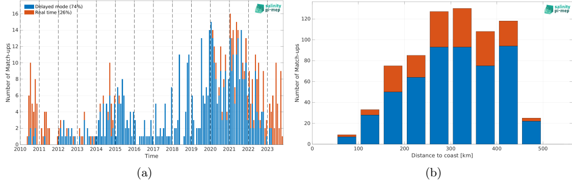
Figure 1: Number of match-ups between Argo and SMOS SSS L2Q v331 - 0.25 Deg (CATDS-CPDC) SSS as a function of time (a) and as function of the distance to coast (b) over the Mississippi river plume Pi-MEP region and for the full satellite product period.
