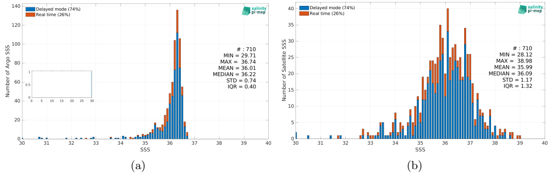
Figure 2: Histograms of SSS from Argo (a) and SMOS SSS L2Q v331 - 0.25 Deg (CATDS-CPDC) (b) considering all match-up pairs per bins of 0.1 over the Mississippi river plume Pi-MEP region and for the full satellite product period.
