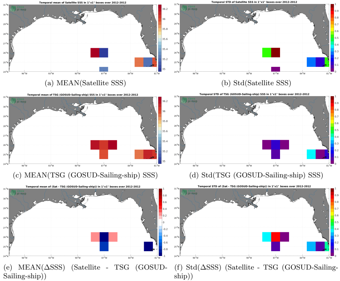
Figure 6: Temporal mean (left) and Std (right) of SSS from SMOS SSS L2Q v330 - 0.25 Deg (CATDS-CPDC) (top), TSG (GOSUD-Sailing-ship) (middle), and of \Delta\text{SSS} (Satellite - TSG (GOSUD-Sailing-ship)). Only match-up pairs are used to generate these maps.
