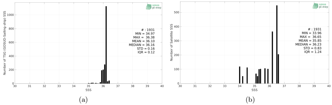
Figure 2: Histograms of SSS from TSG (GOSUD-Sailing-ship) (a) and SMOS SSS L2Q v330 - 0.25 Deg (CATDS-CPDC) (b) considering all match-up pairs per bins of 0.1 over the Mississippi river plume Pi-MEP region and for the full satellite product period.
