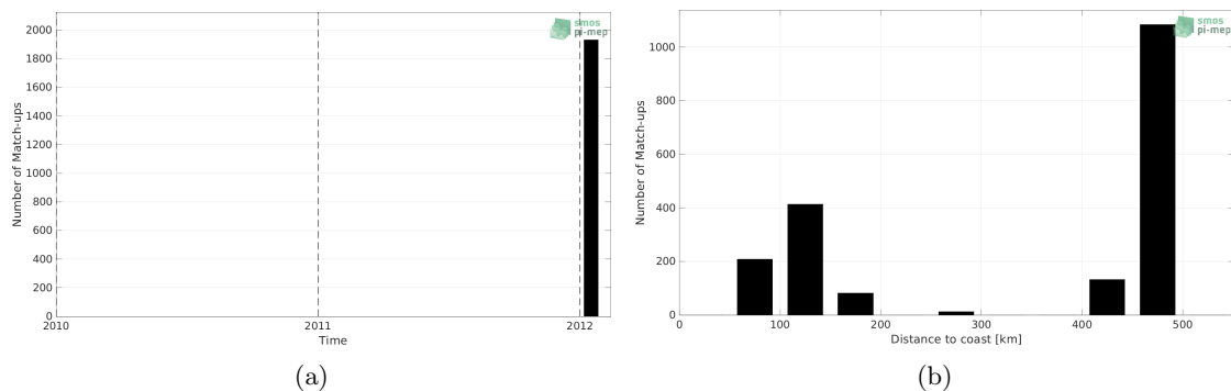
Figure 1: Number of match-ups between TSG (GOSUD-Sailing-ship) and SMOS SSS L2Q v330 - 0.25 Deg (CATDS-CPDC) SSS as a function of time (a) and as function of the distance to coast (b) over the Mississippi river plume Pi-MEP region and for the full satellite product period.
