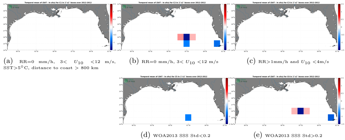
Figure 12: Temporal mean gridded over spatial boxes of size 1^{\circ}\times 1^{\circ} of \Delta SSS (SMOS SSS L2Q v330 - 0.25 Deg (CATDS-CPDC) - TSG (GOSUD-Sailing-ship)) for 5 different subdatasets corresponding to:RR=0 mm/h, 3 < U_{10} < 12 m/s, SST >5^{\circ}\text{C} , distance to coast > 800 km (a), RR=0 mm/h, 3 < U_{10} < 12 m/s (b), RR >1 mm/h and U_{10} < 4 m/s (c), WOA2013 SSS Std <0.2 (d), WOA2013 SSS Std >0.2 (e).
