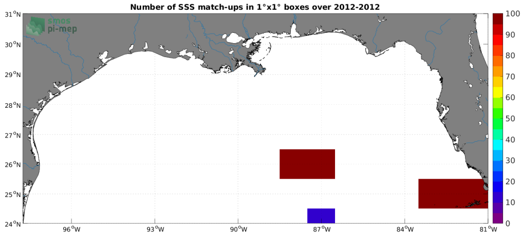
Figure 4: Number of SSS match-ups between TSG (GOSUD-Sailing-ship) SSS and the SMOS SSS L2Q v330 - 0.25 Deg (CATDS-CPDC) SSS product for the Mississippi river plume Pi-MEP region over 1^\circ \times 1^\circ boxes and for the full satellite product period.
