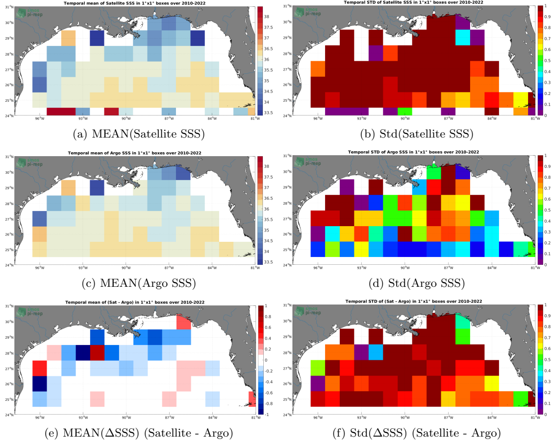
Figure 6: Temporal mean (left) and Std (right) of SSS from SMOS SSS L2Q v330 - 0.25 Deg (CATDS-CPDC) (top), Argo (middle), and of \Delta\text{SSS} (Satellite - Argo). Only match-up pairs are used to generate these maps.
