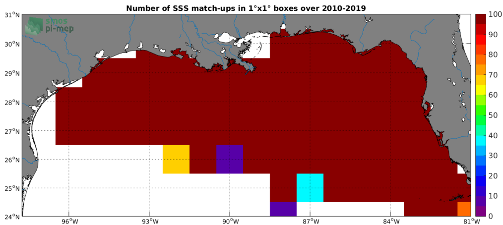
Figure 4: Number of SSS match-ups between TSG-SAMOS SSS and the SMOS L2Q v321 - 0.25 Deg (CATDS-CPDC) SSS product for the Mississippi river plume Pi-MEP region over 1^\circ \times 1^\circ boxes and for the full satellite product period.
