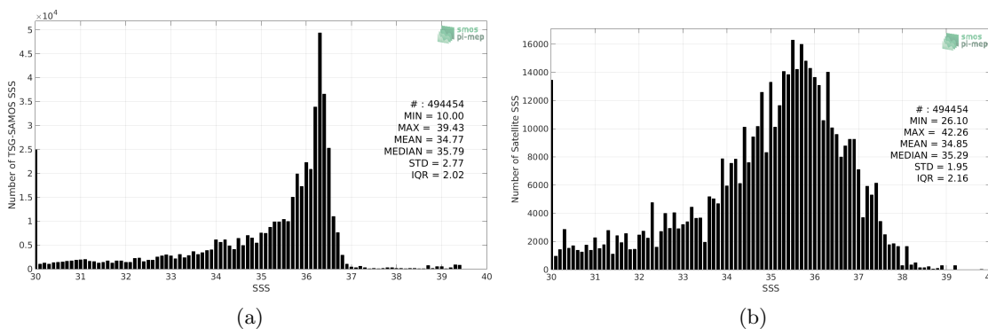
Figure 2: Histograms of SSS from TSG-SAMOS (a) and SMOS L2Q v321 - 0.25 Deg (CATDS-CPDC) (b) considering all match-up pairs per bins of 0.1 over the Mississippi river plume Pi-MEP region and for the full satellite product period.
