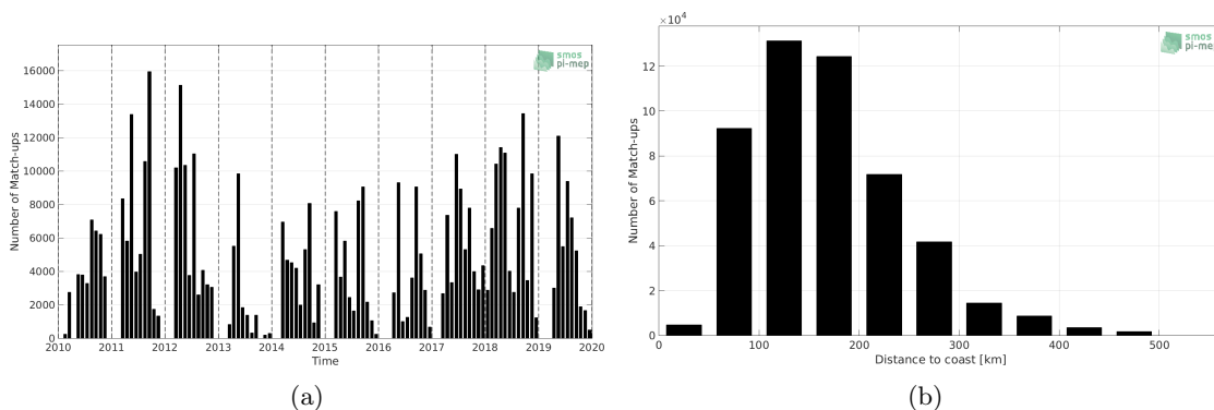
Figure 1: Number of match-ups between TSG-SAMOS and SMOS L2Q v321 - 0.25 Deg (CATDS-CPDC) SSS as a function of time (a) and as function of the distance to coast (b) over the Mississippi river plume Pi-MEP region and for the full satellite product period.
