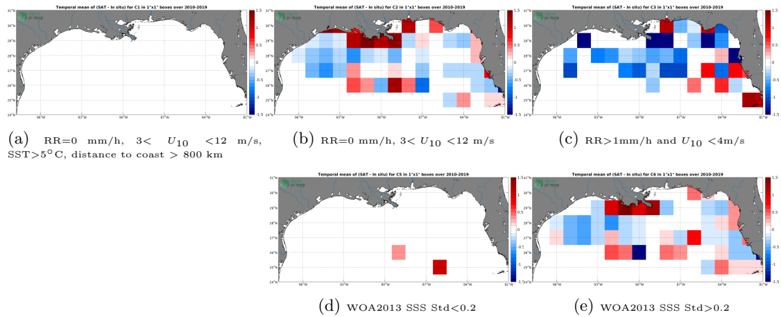
Figure 12: Temporal mean gridded over spatial boxes of size 1^{\circ}\times 1^{\circ} of \Delta\text{SSS} (SMOS L2Q v321 - 0.25 Deg (CATDS-CPDC) - TSG-SAMOS) for 5 different subdatasets corresponding to:RR=0 mm/h, 3 < U_{10} < 12 m/s, SST >5^{\circ}\text{C} , distance to coast > 800 km (a), RR=0 mm/h, 3 < U_{10} < 12 m/s (b), RR >1 mm/h and U_{10} < 4 m/s (c), WOA2013 SSS Std <0.2 (d), WOA2013 SSS Std >0.2 (e).
