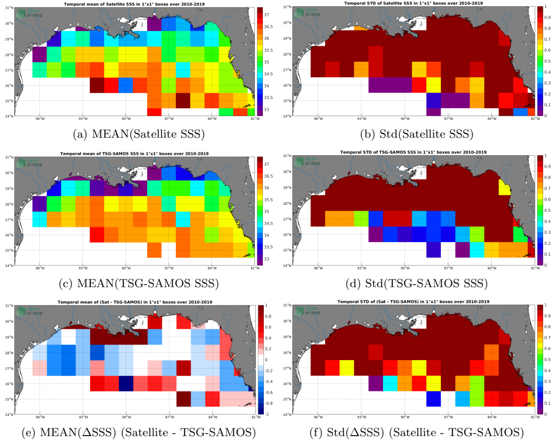
Figure 6: Temporal mean (left) and Std (right) of SSS from SMOS L2Q v321 - 0.25 Deg (CATDS-CPDC) (top), TSG-SAMOS (middle), and of \Delta SSS (Satellite - TSG-SAMOS). Only match-up pairs are used to generate these maps.
