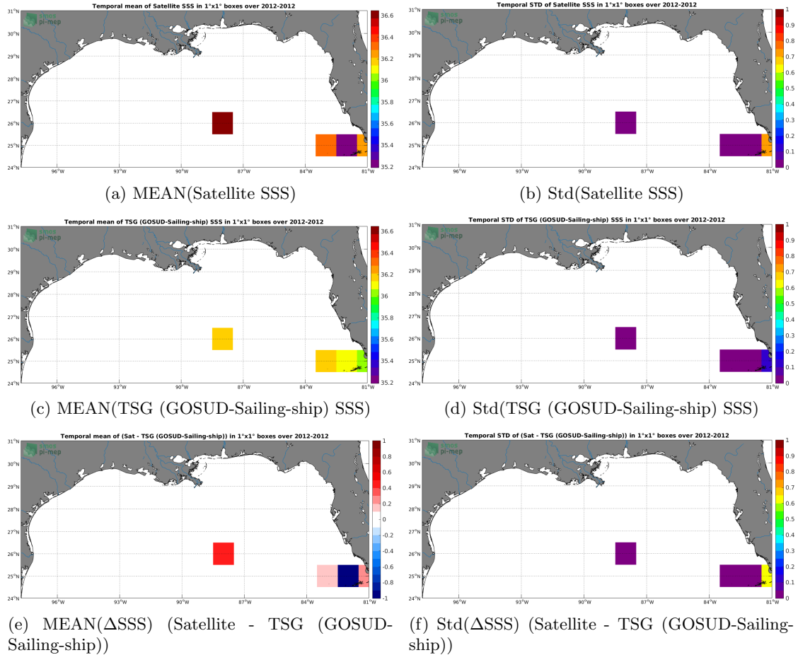
Figure 6: Temporal mean (left) and Std (right) of SSS from SMOS SSS L2Q v321 - 0.25 Deg (CATDS-CPDC) (top), TSG (GOSUD-Sailing-ship) (middle), and of \Delta\text{SSS} (Satellite - TSG (GOSUD-Sailing-ship)). Only match-up pairs are used to generate these maps.
